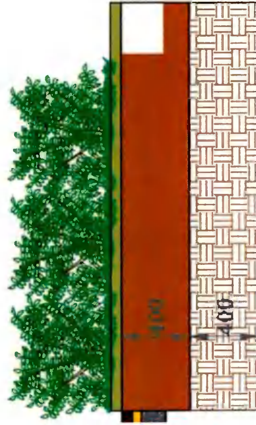
Depth of soil in shrub planting areas
