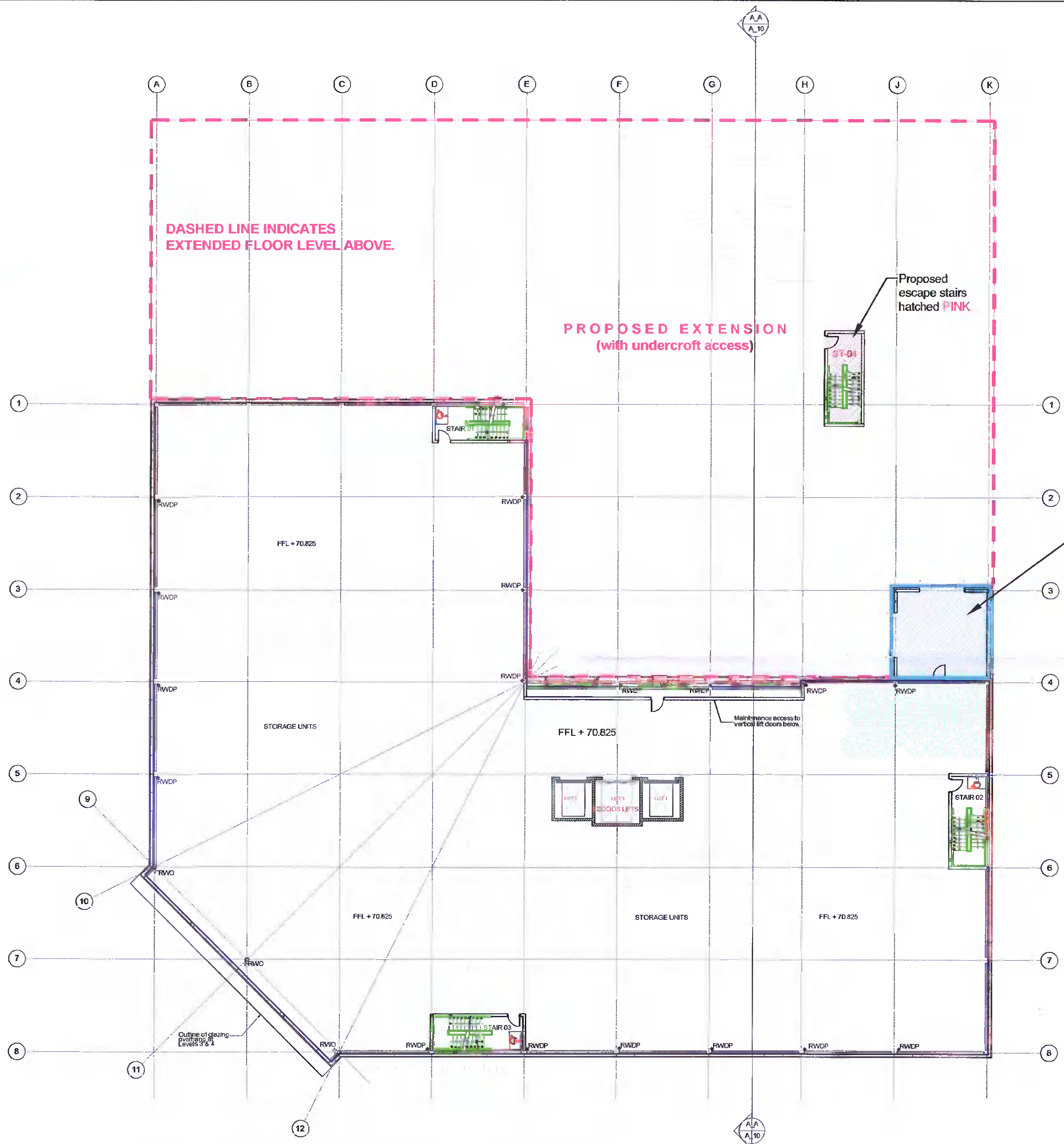
First Floor Plan (Scale 1:250).
