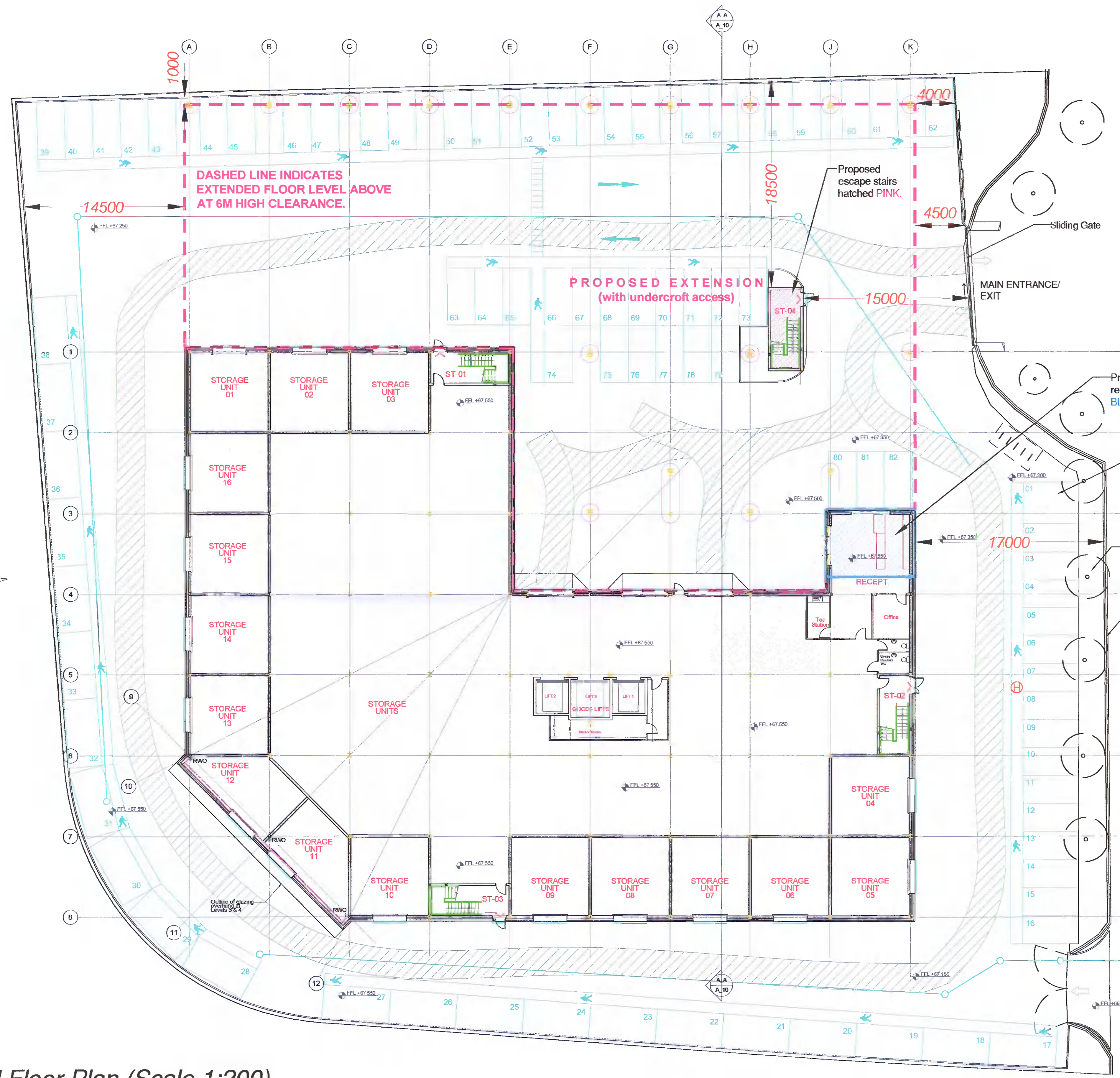
Ground Floor Plan (Scale 1:200).
