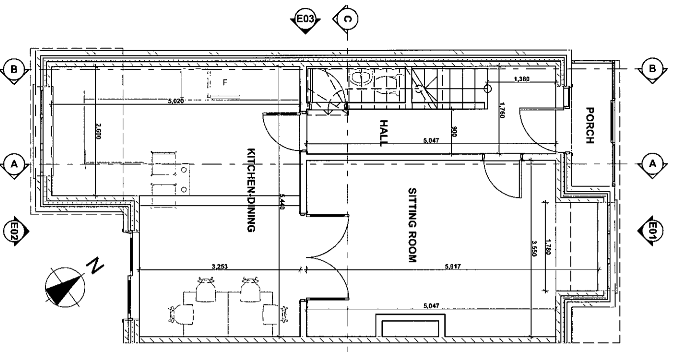
Ground Floor Plan (Existing) 1:75
