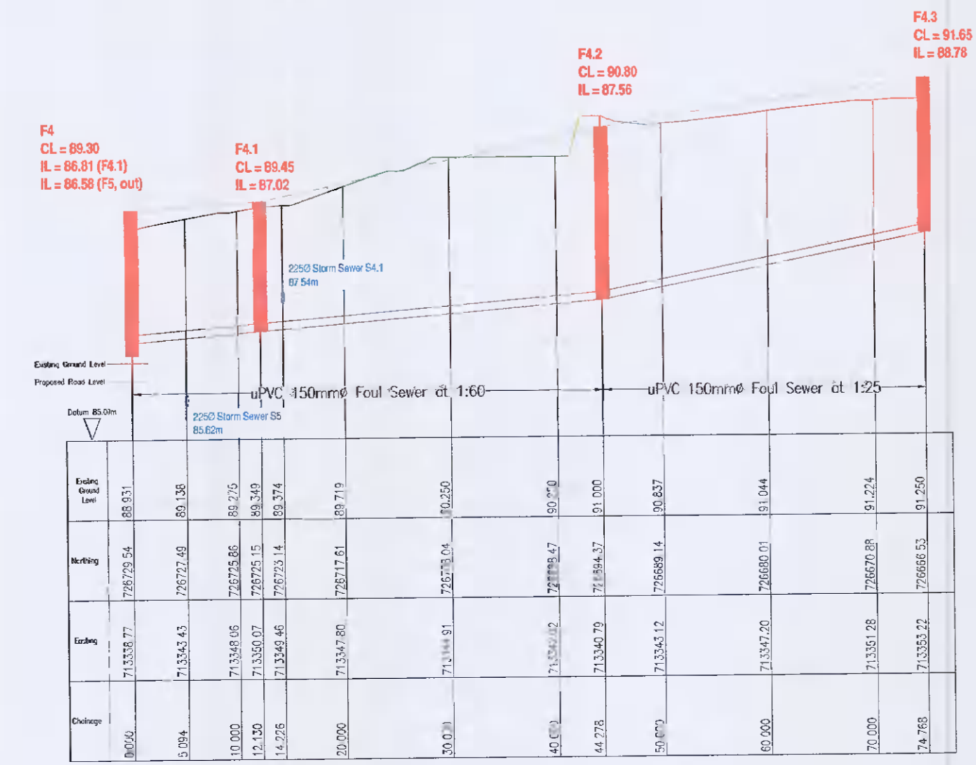
FOUL SEWER F4 TO F4.3 LONGITUDINAL SECTION Scale 1:500 Horizontal, 1:100 Vertical
