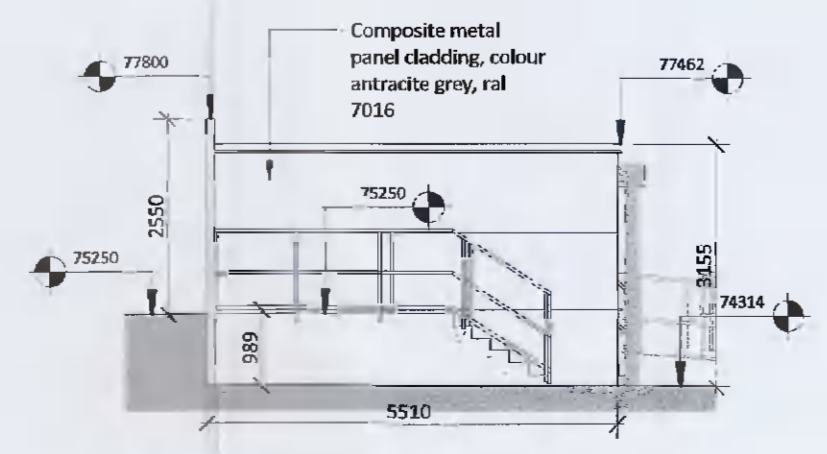
6 Waste Compound - West Elevation 1 : 100
