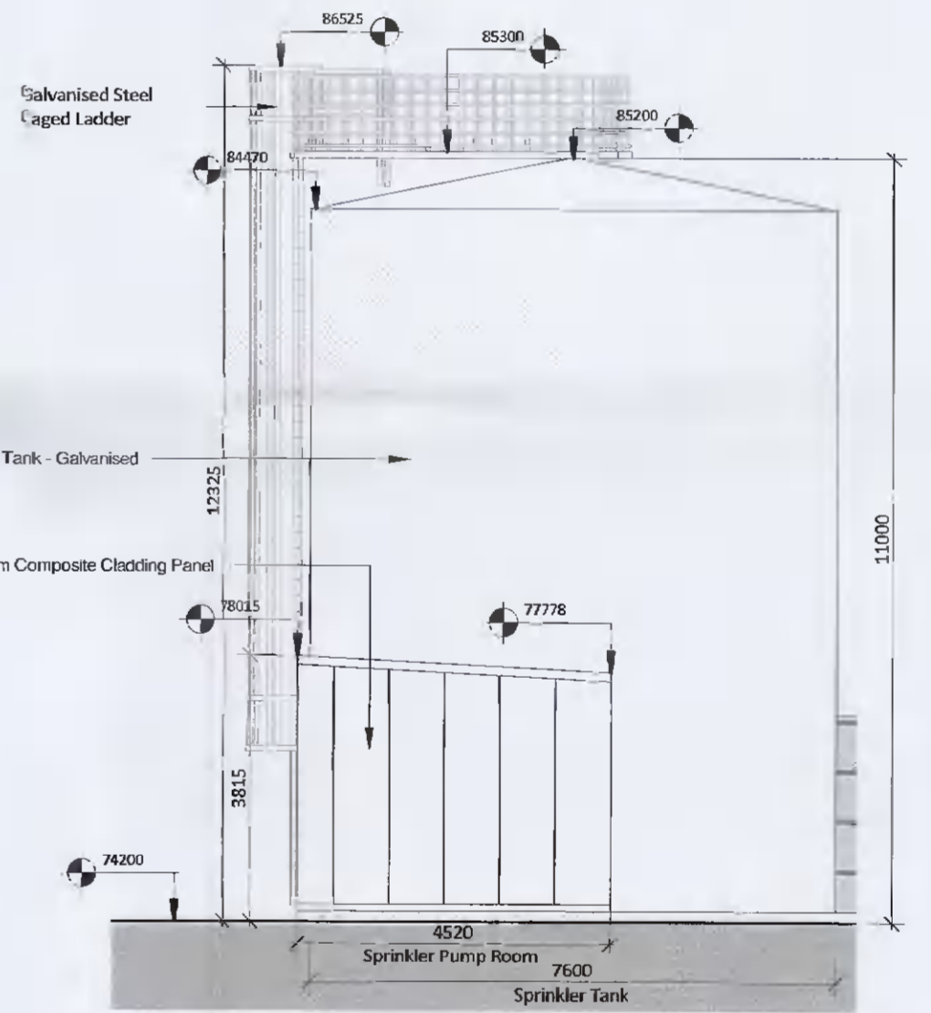
10 Sprinkler Plant - West Elevation 1 : 100
