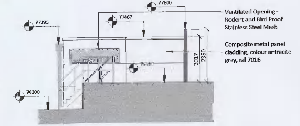
5 Waste Compound - East Elevation 1 : 100
