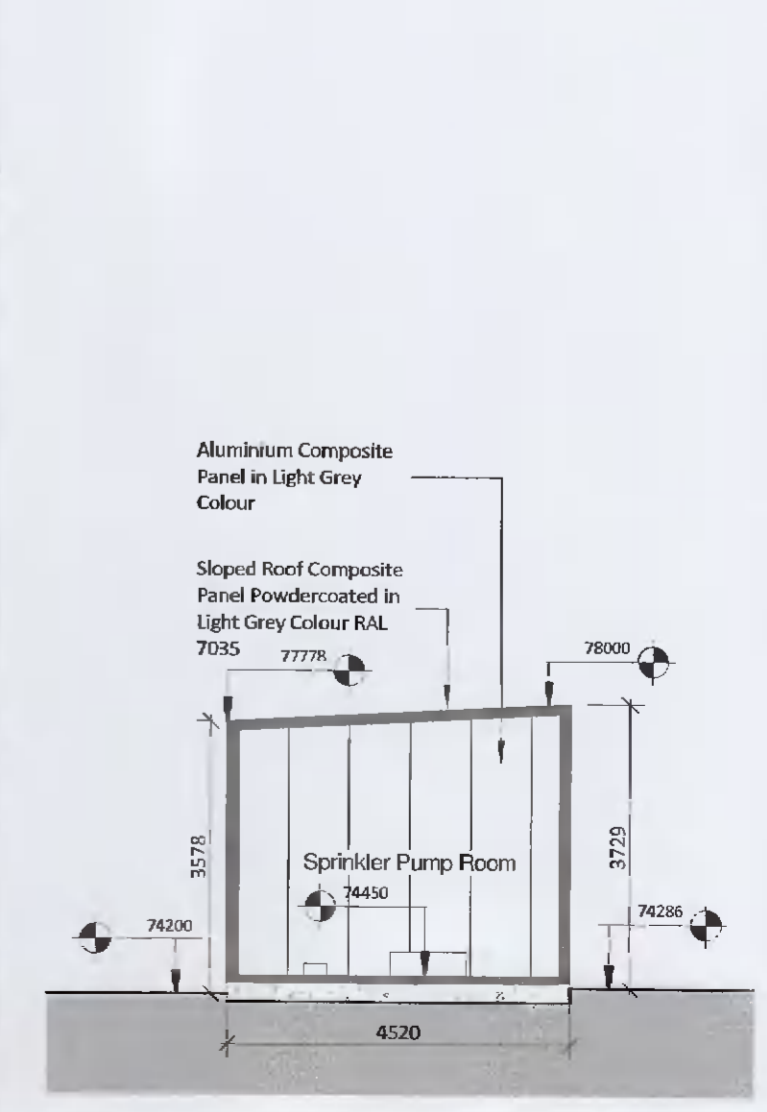
12 Sprinkler Plant - Section 1 : 100
