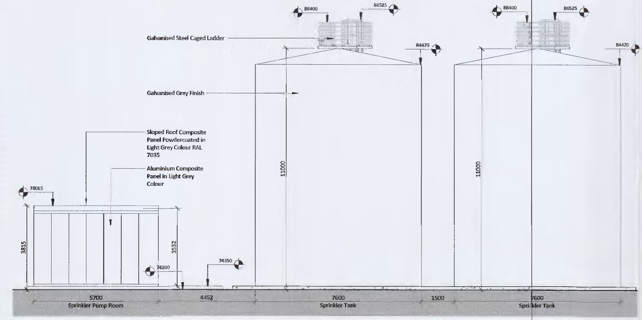
11 Sprinkler Plant - South Elevation 1 : 100
