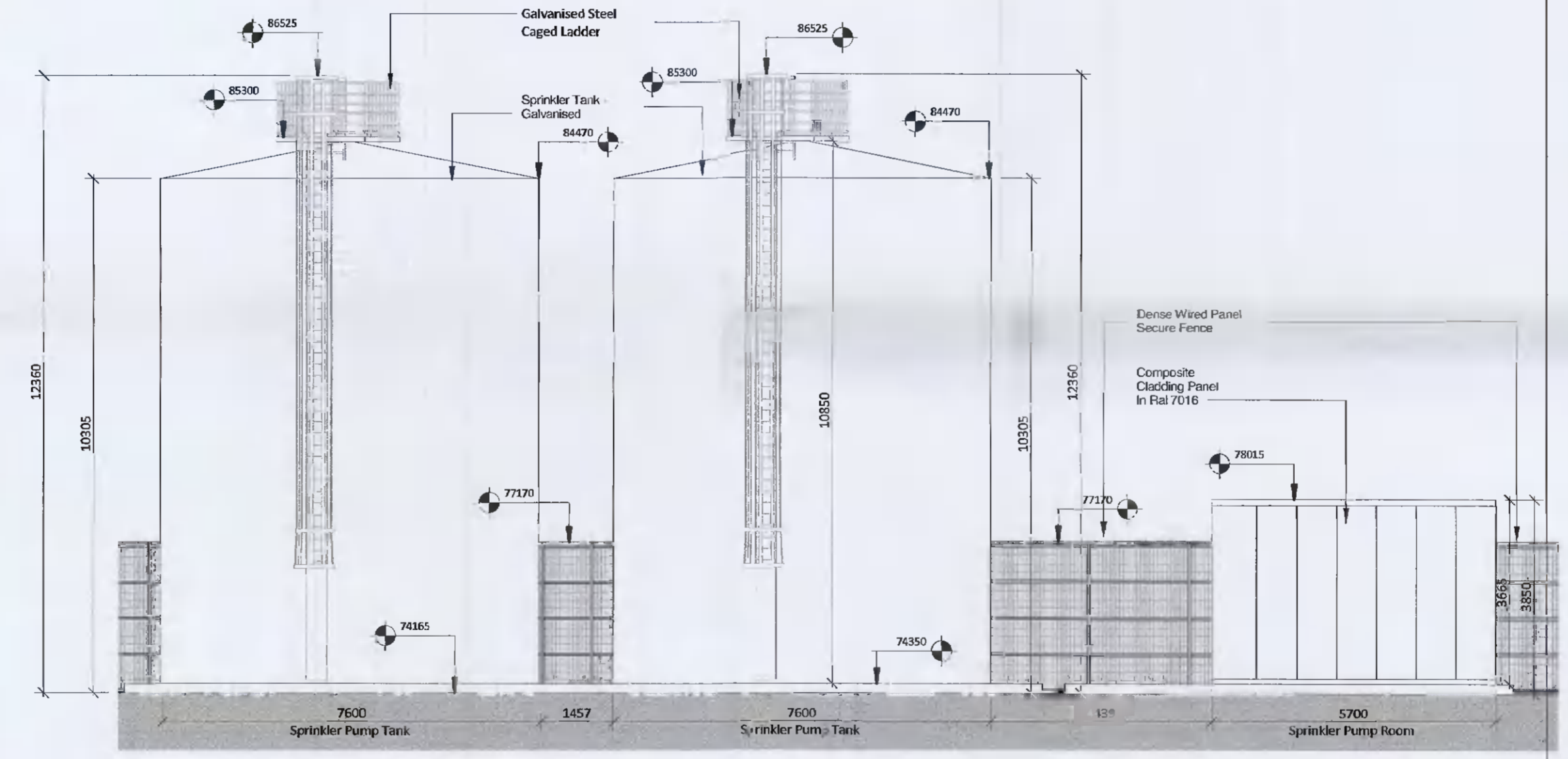
9 Sprinkler Plant - North Elevation 1 : 100
