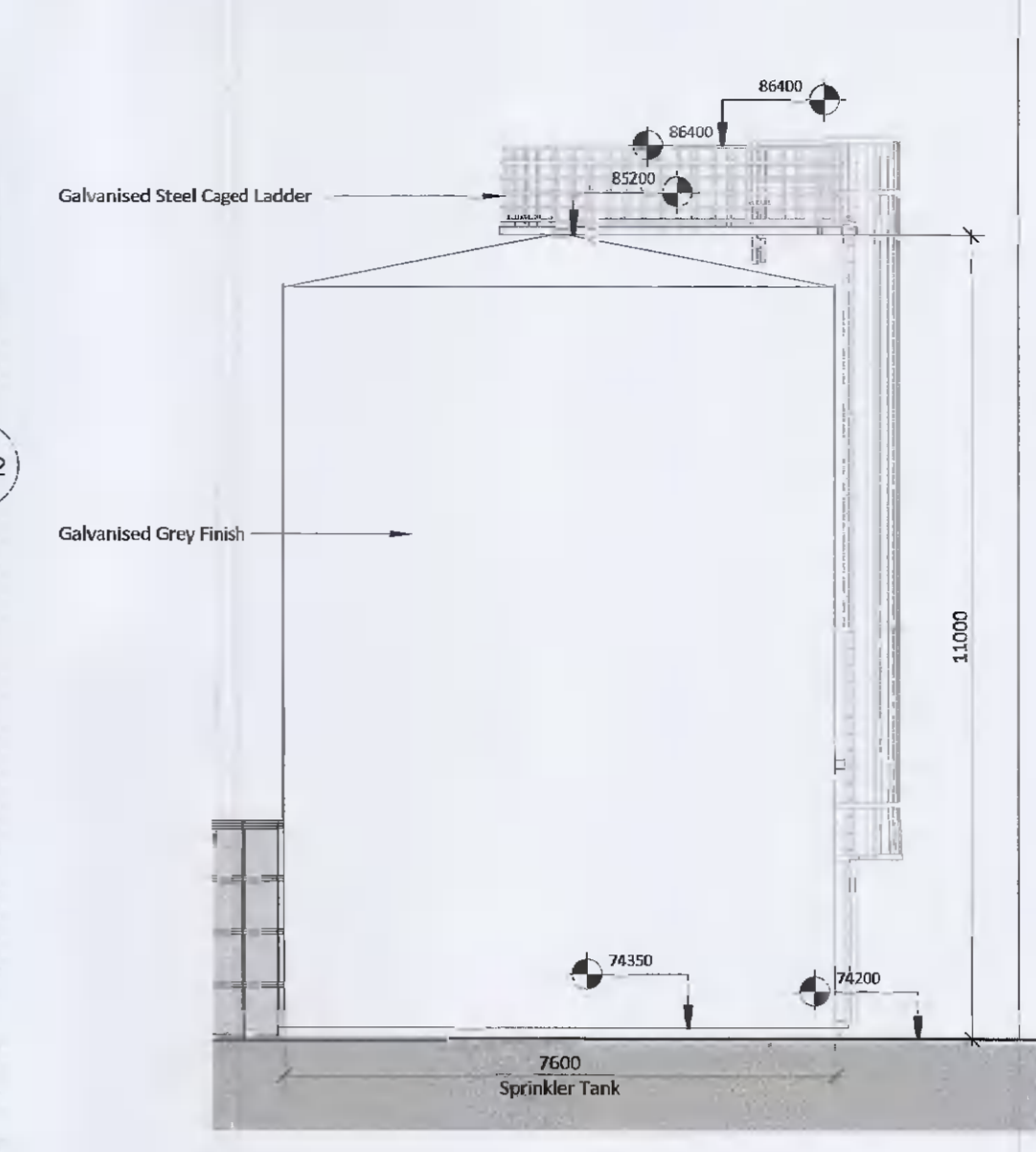
8 Sprinkler Plant - East Elevation 1 : 100
