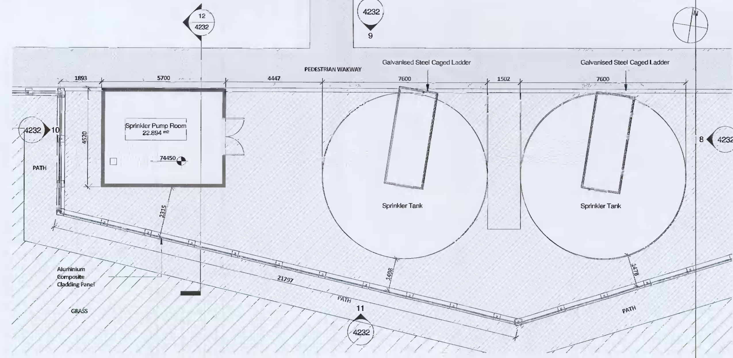
7 Sprinkler Pump Room Plan 1 : 100
