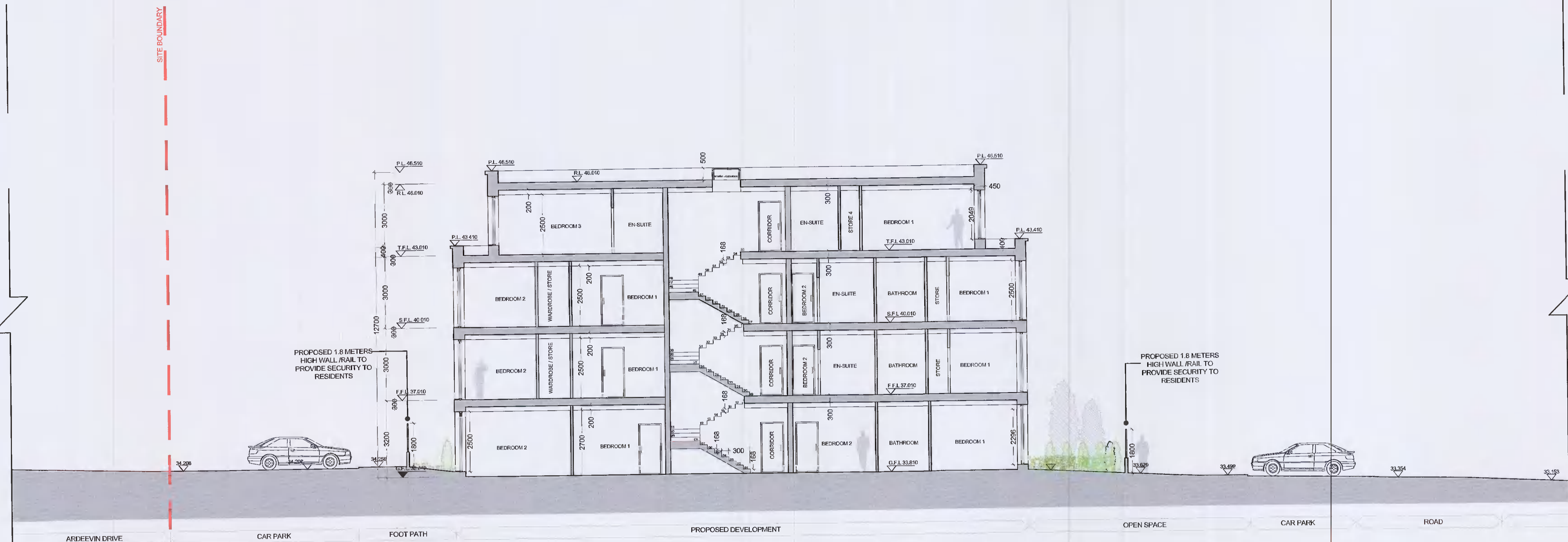
PROPOSED SECTION C-C BALL ALLEY HOUSE, LUCAN, CO. DUBLIN Scale 1:100
