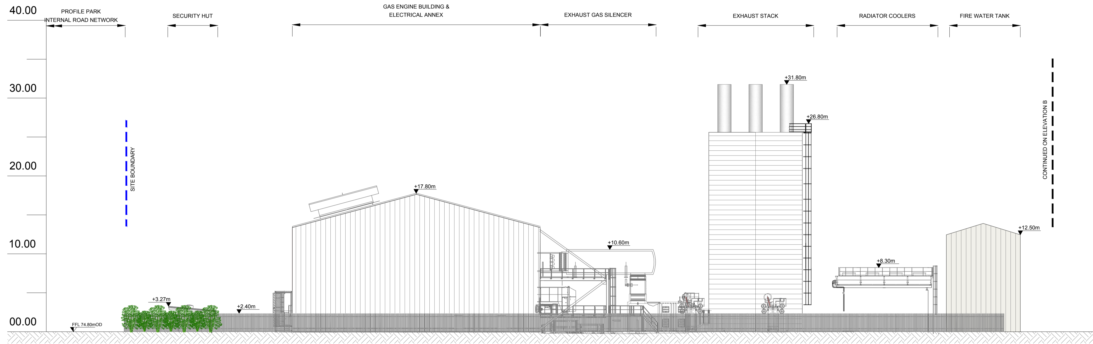
CONTIGUOUS ELEVATION A - Scale 1:250
