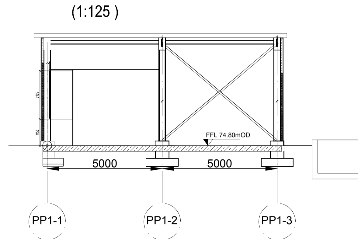
Section S2
