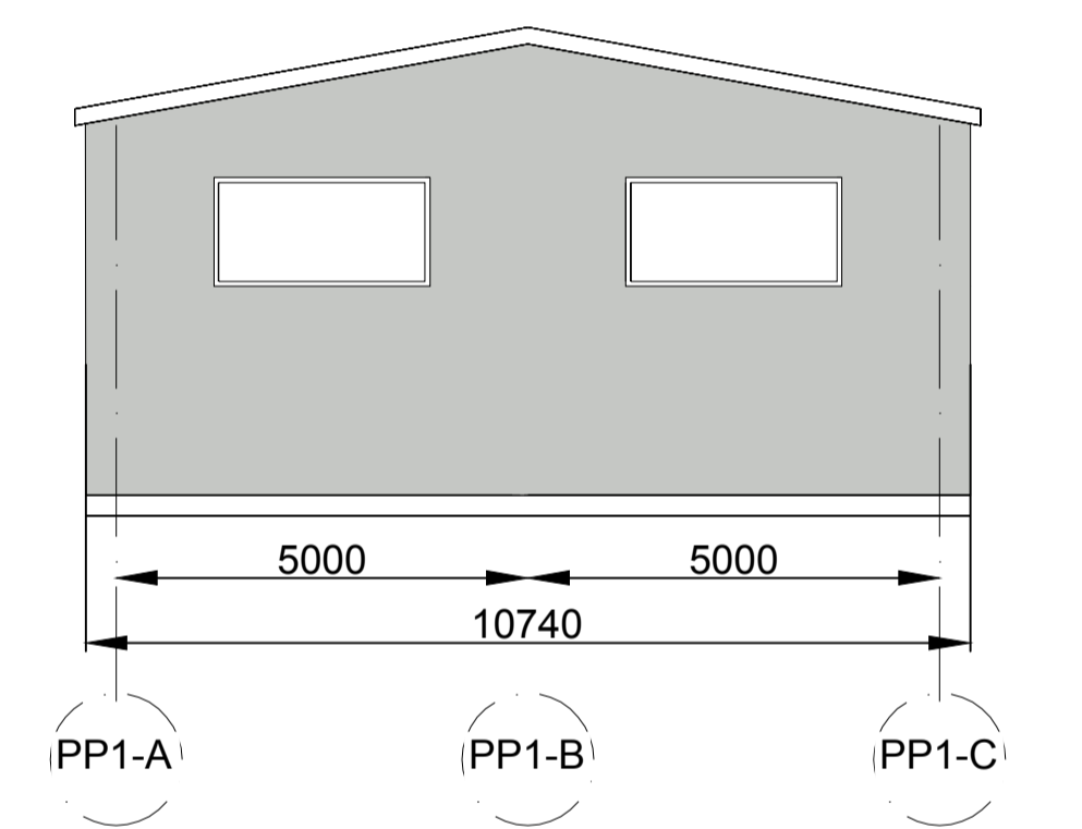
Elevation S3
