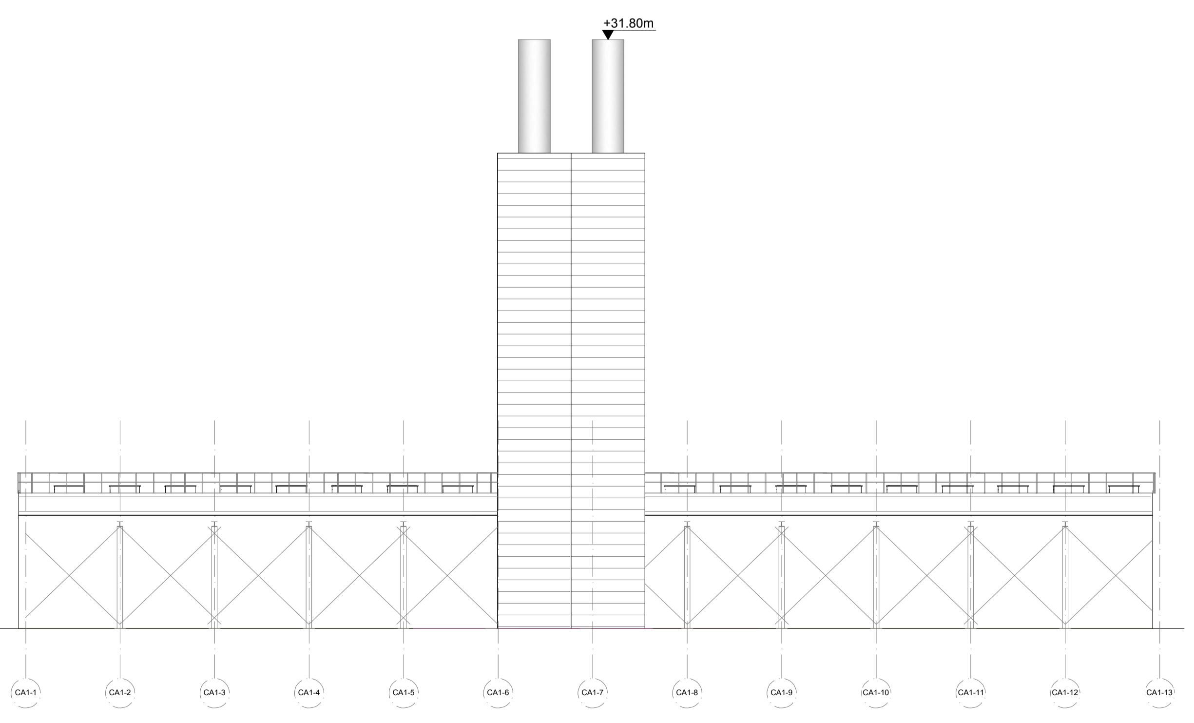
ELEVATION D Scale 1:200
