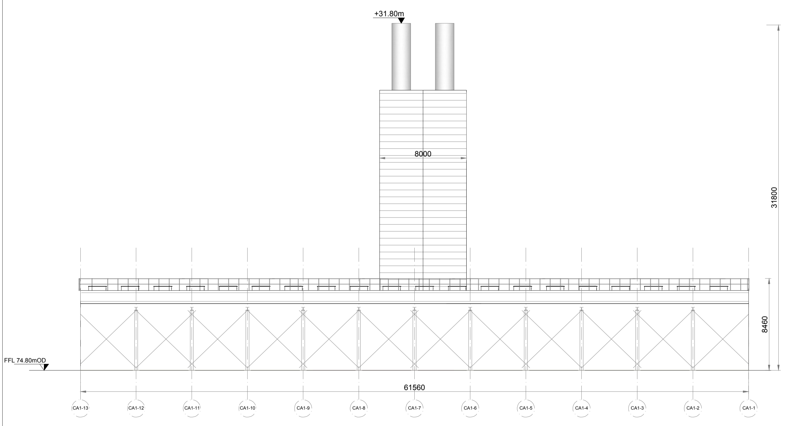
ELEVATION C Scale 1:200
