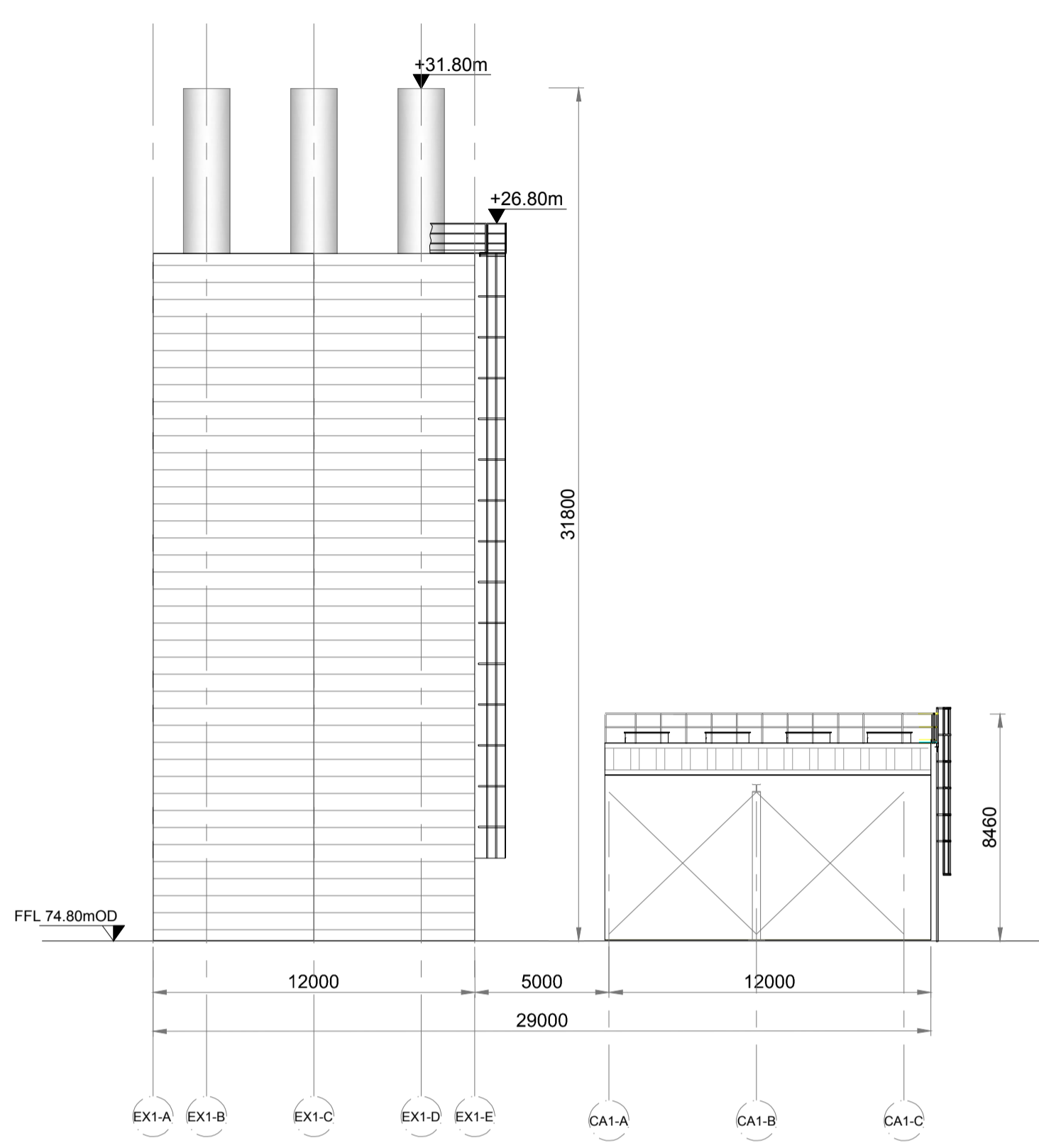
ELEVATION B Scale 1:200
