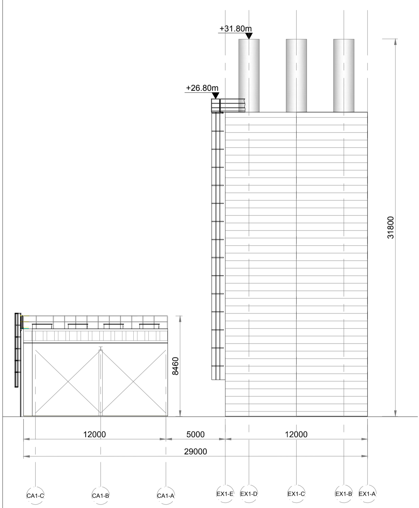
ELEVATION A Scale 1:200
