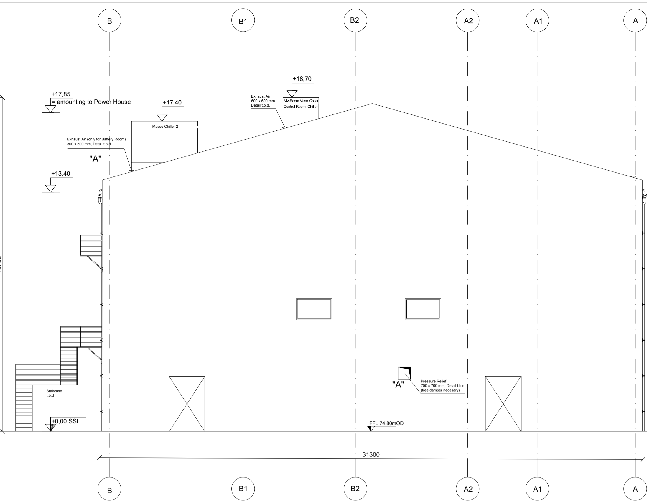
SIDE ELEVATION (Powerhouse Side) Scale 1:125
