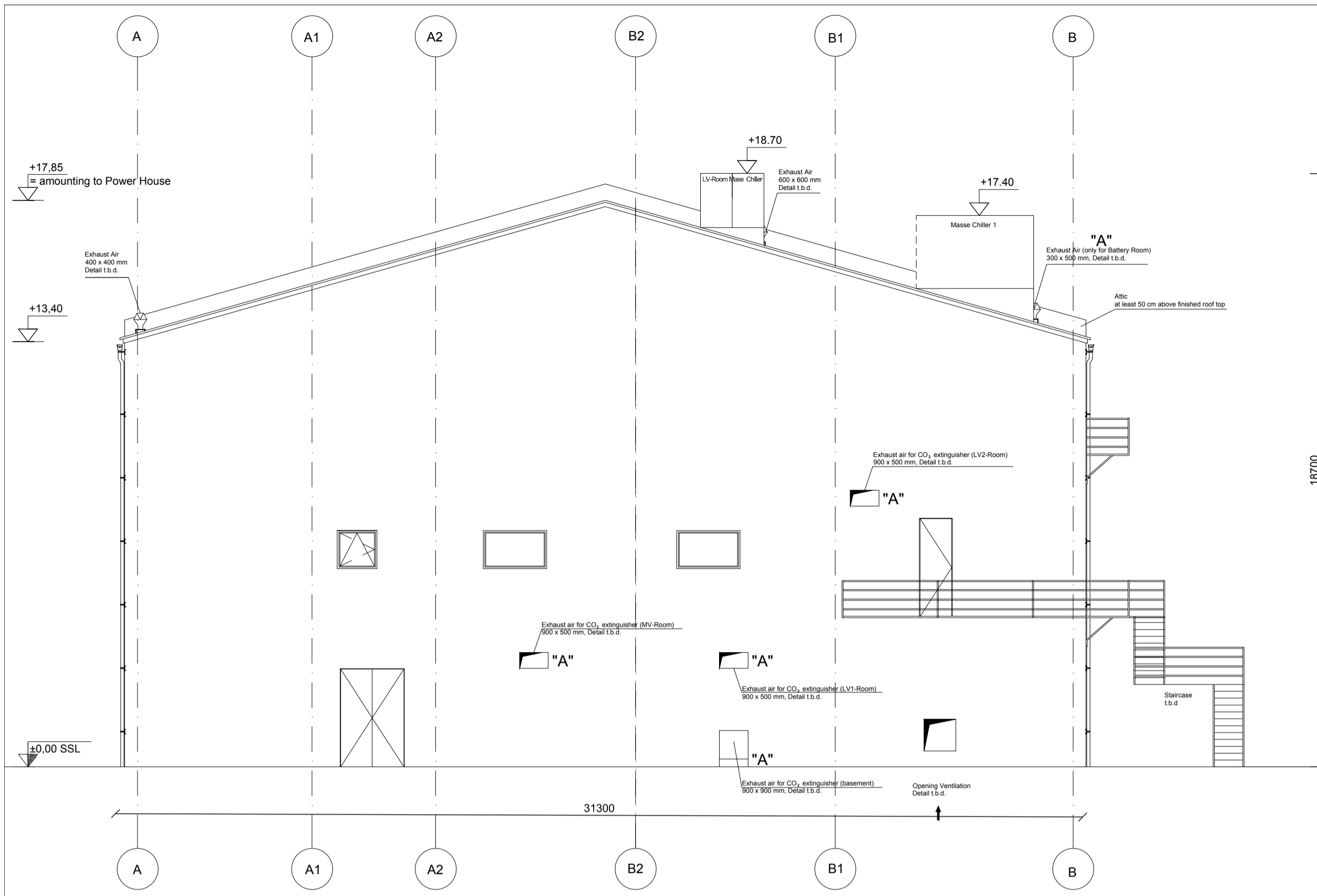
SIDE ELEVATION Scale 1:125
