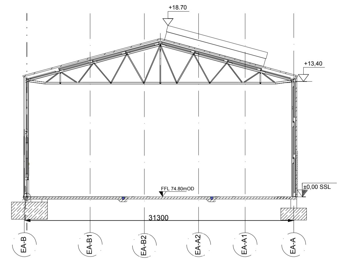
SECTION 1-1 Scale 1:250
