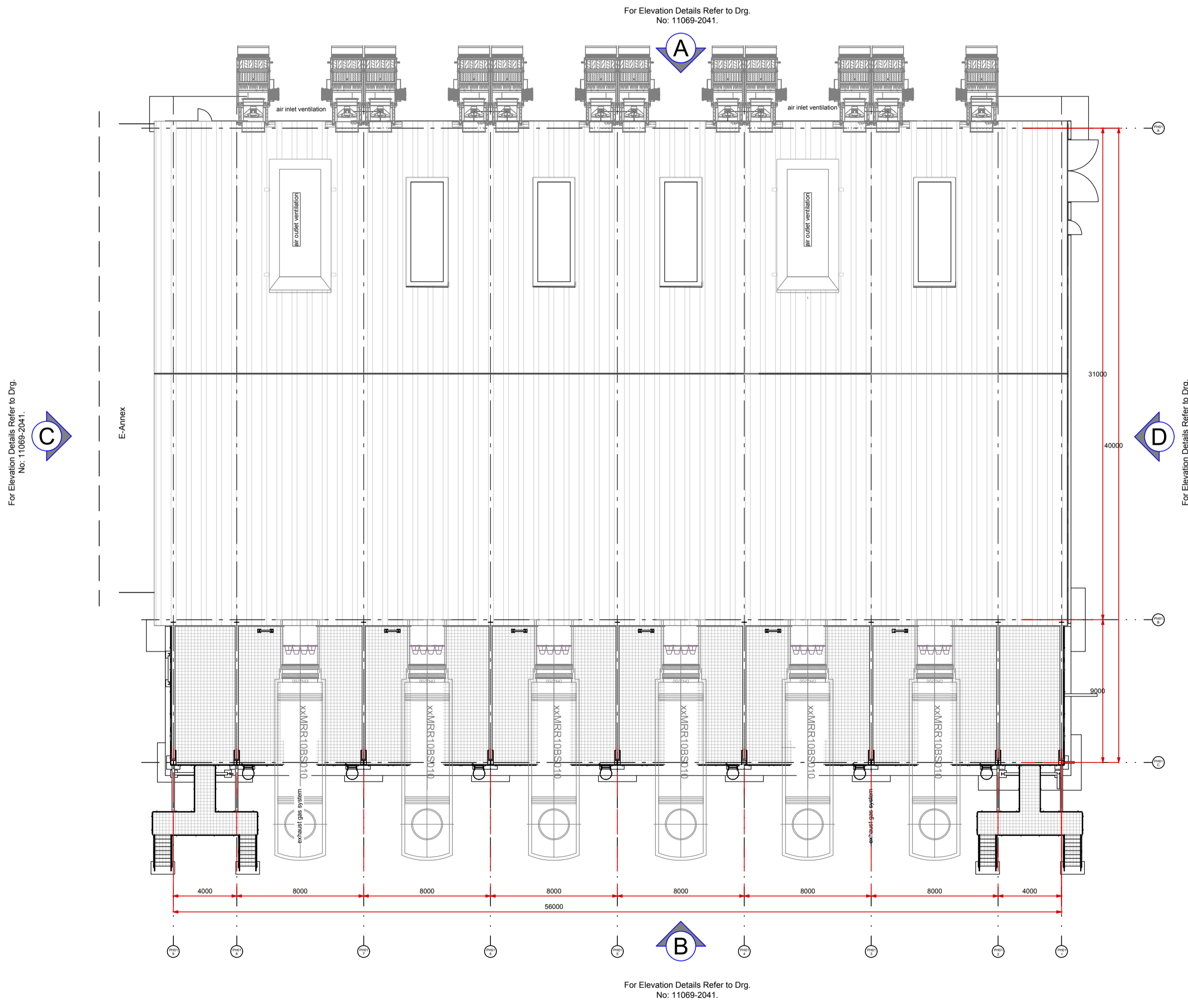
ROOF PLAN
