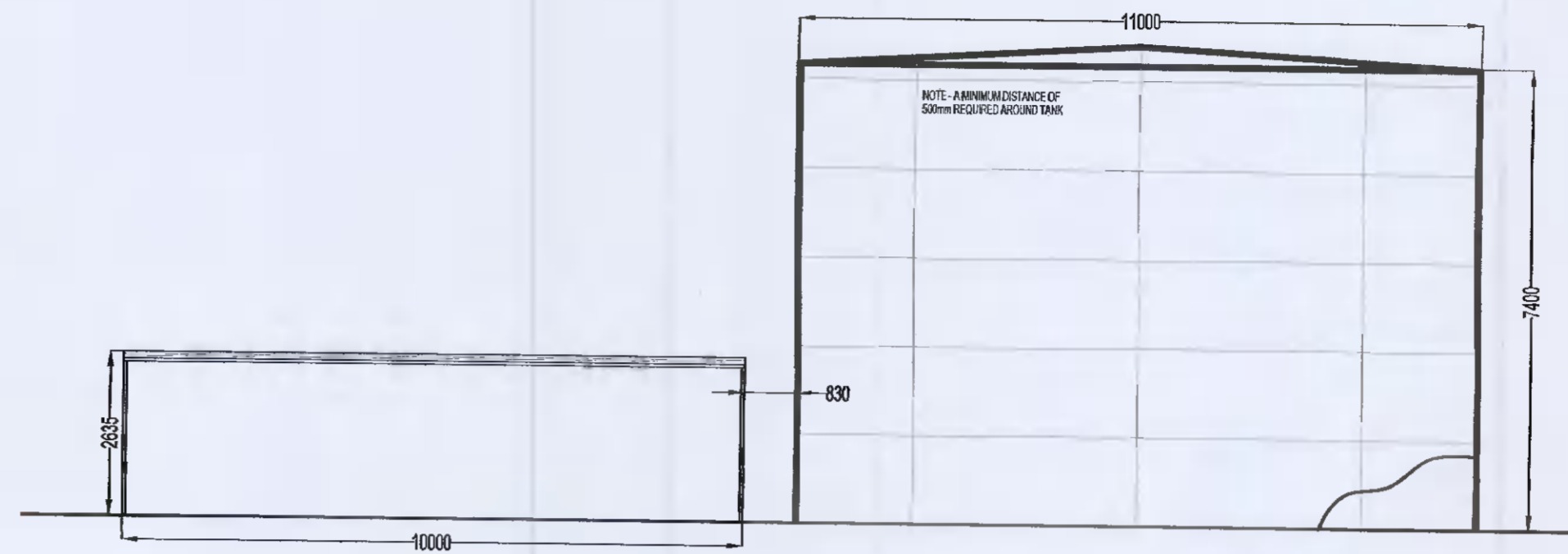
UNIT 1 - SPRINKLER TANK & PUMP HOUSE SECTION A-A SCALE 1:100
