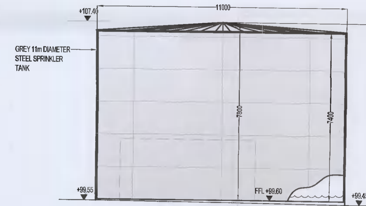
SOUTHERN (SIDE) ELEVATION SCALE 1:100
