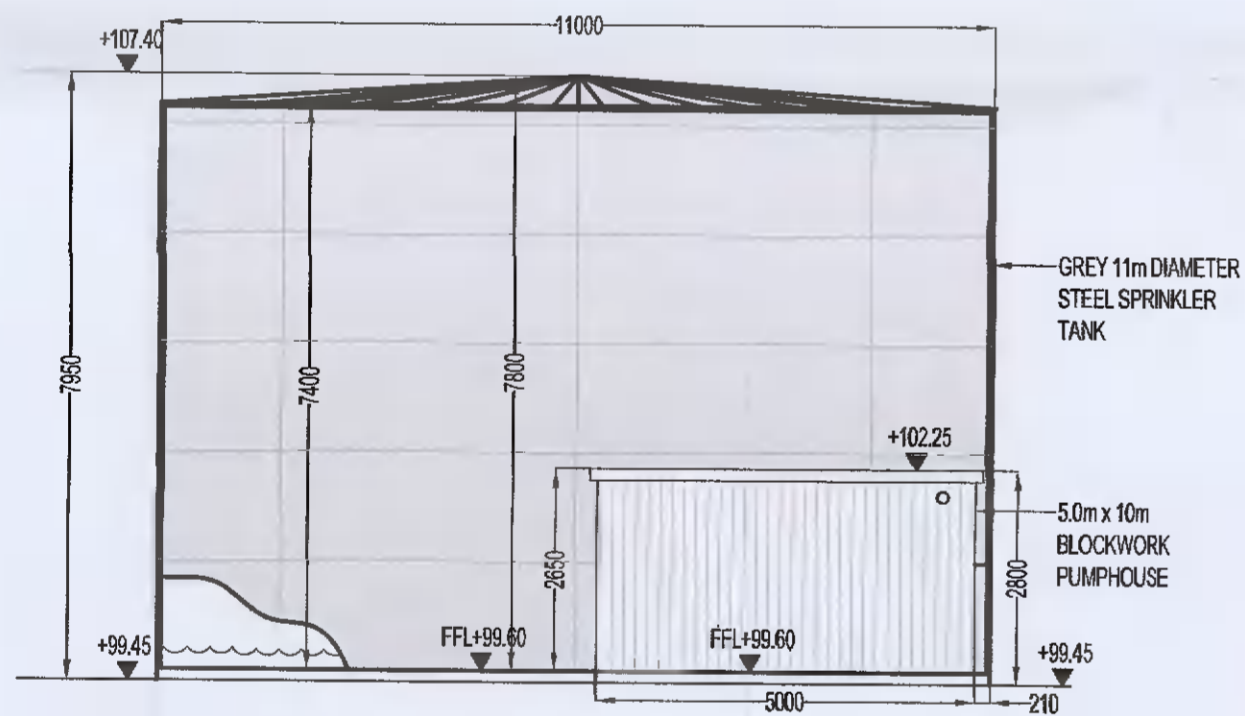
NORTHERN (SIDE) ELEVATION SCALE 1:100
