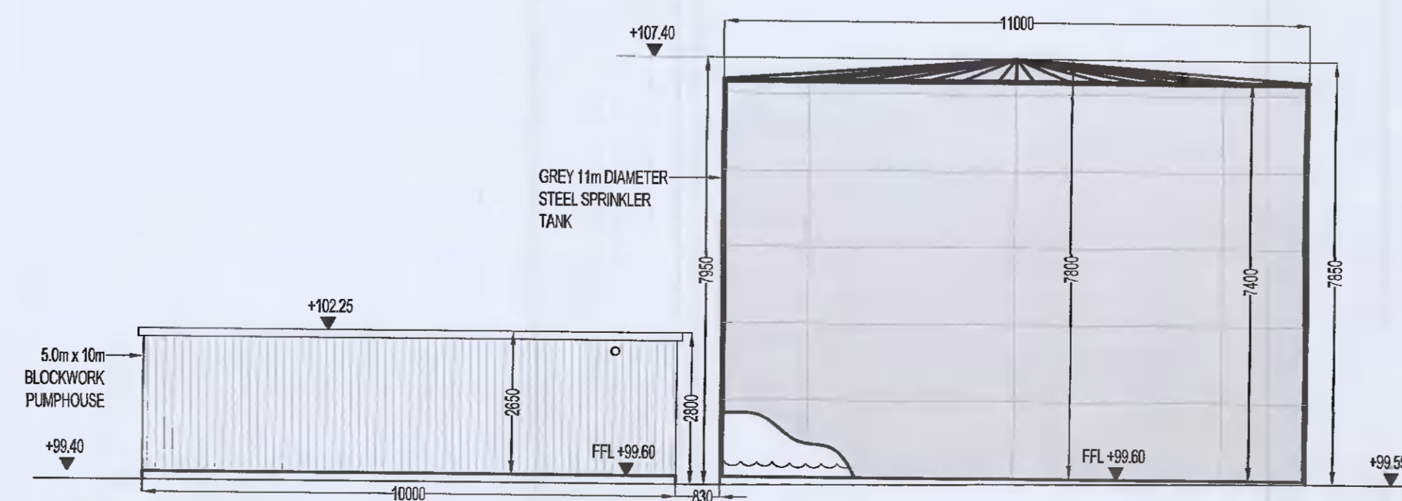
WESTERN (REAR) ELEVATION SCALE 1:100
