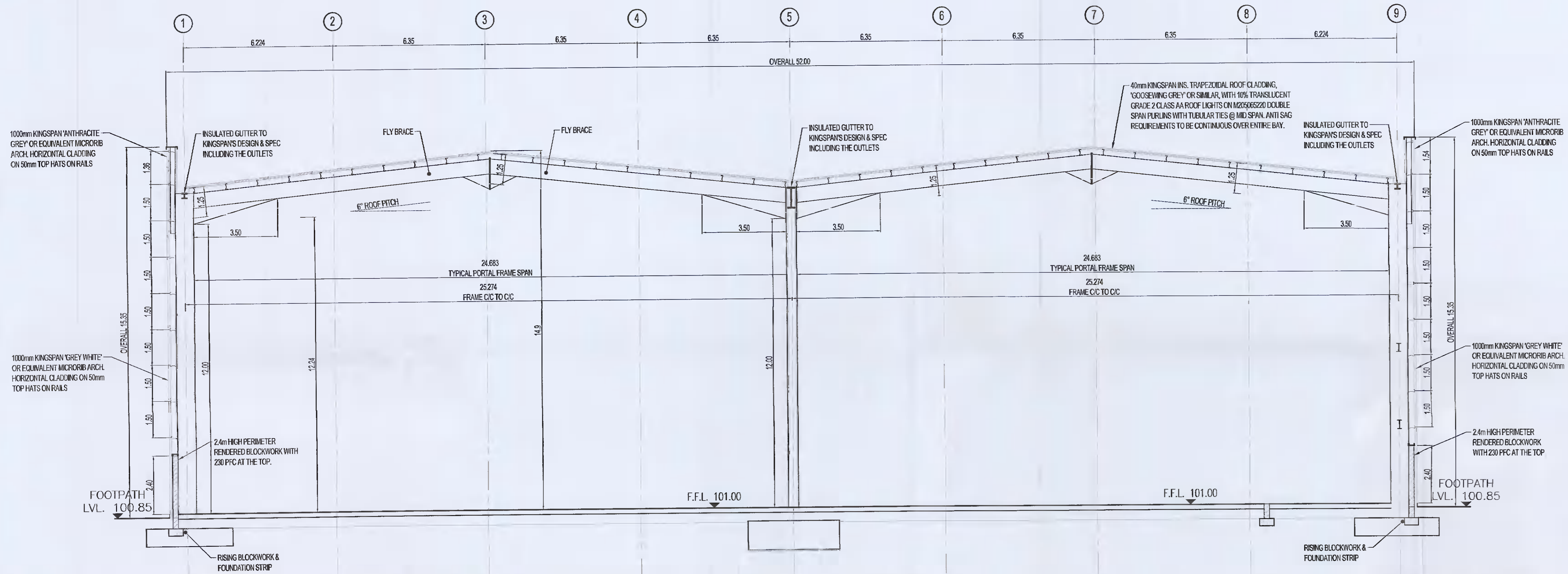
SECTION 2-2 SCALE 1:100
