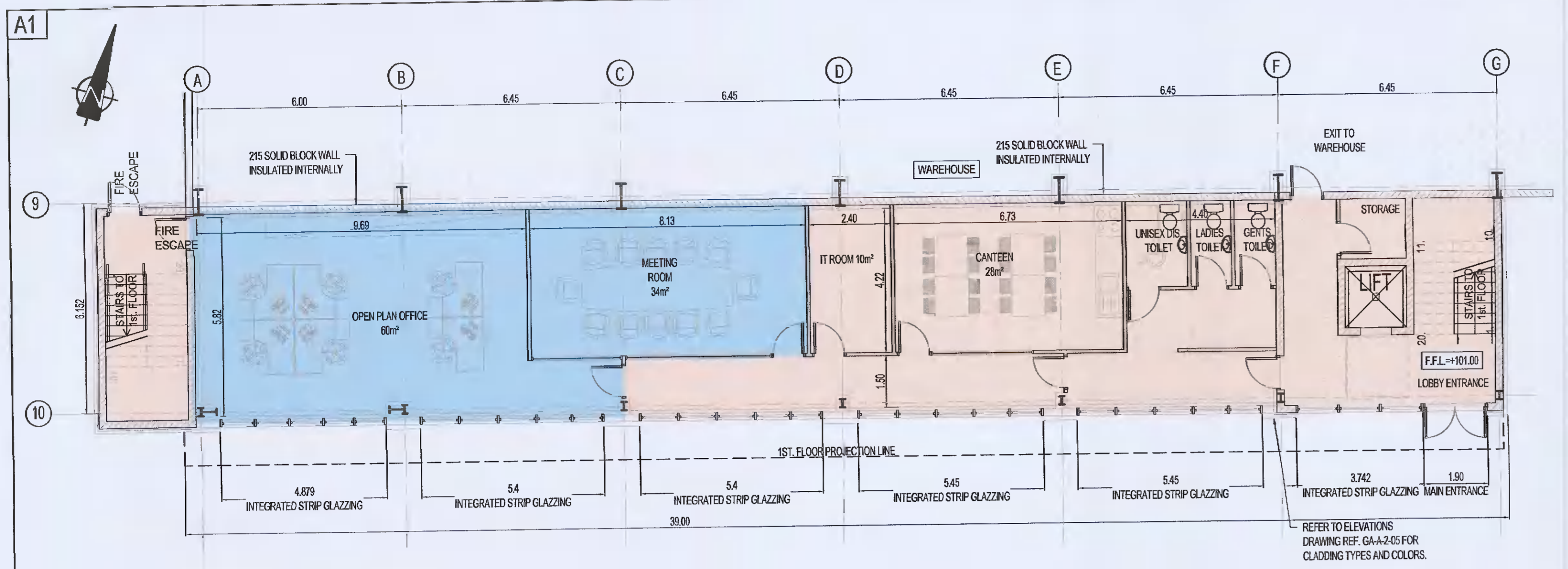
ANCILLARY OFFICES - GROUND FLOOR PLAN SCALE 1:100
