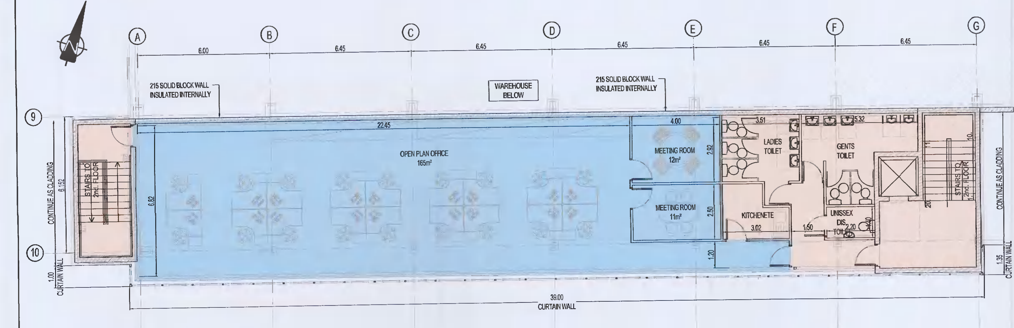
ANCILLARY OFFICES - SECOND FLOOR PLAN SCALE 1:100
