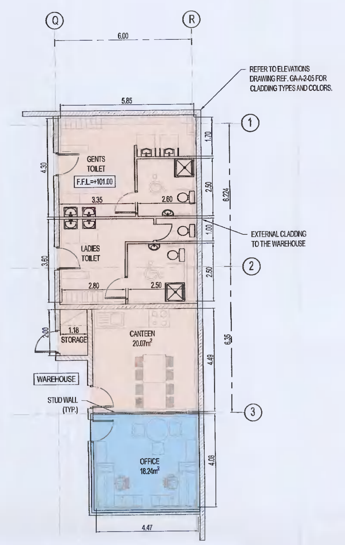
STAFF FACILITIES TOILET BLOCK - GROUND FLOOR PLAN SCALE 1:100
