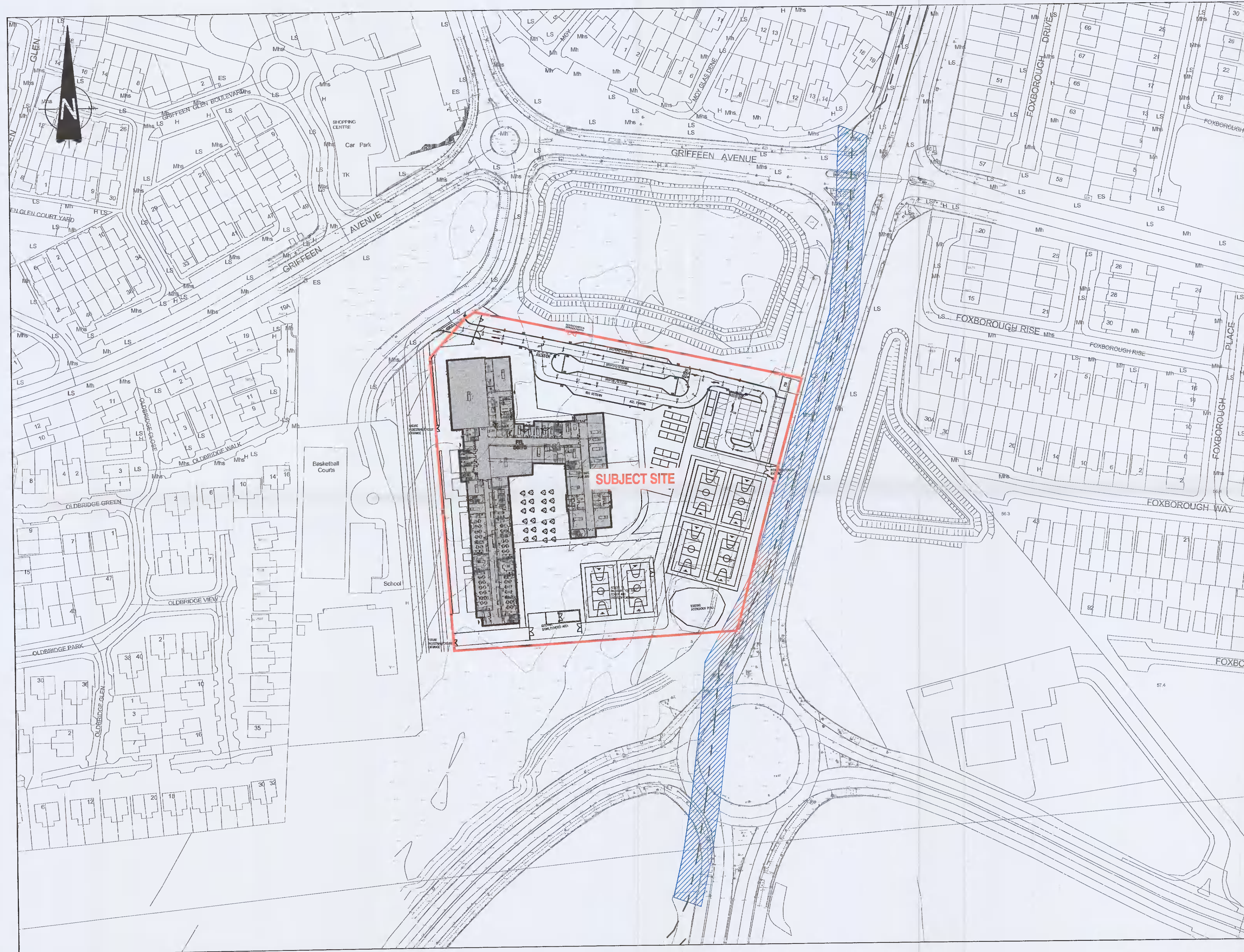
SITE LOCATION PLAN SCALE 1:1000 @ A1
