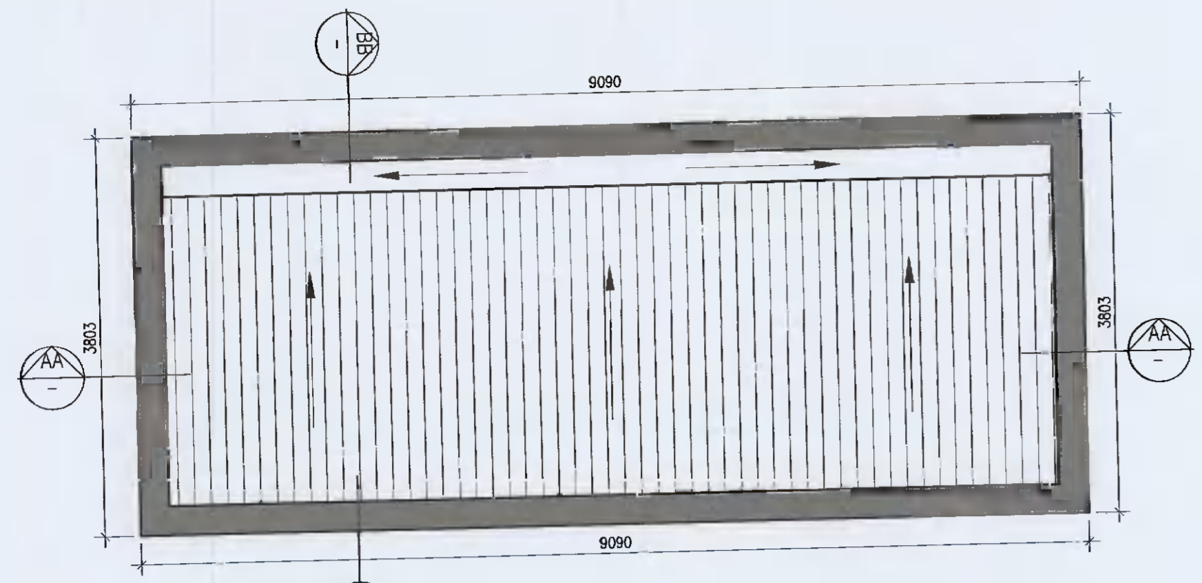
1 Bicycle Store Type 1 Roof Plan Scale 1:50
