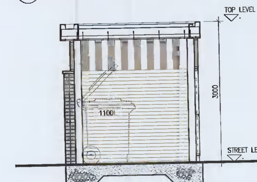
12 Bicycle Store Type 2 Section A Scale 1:50
