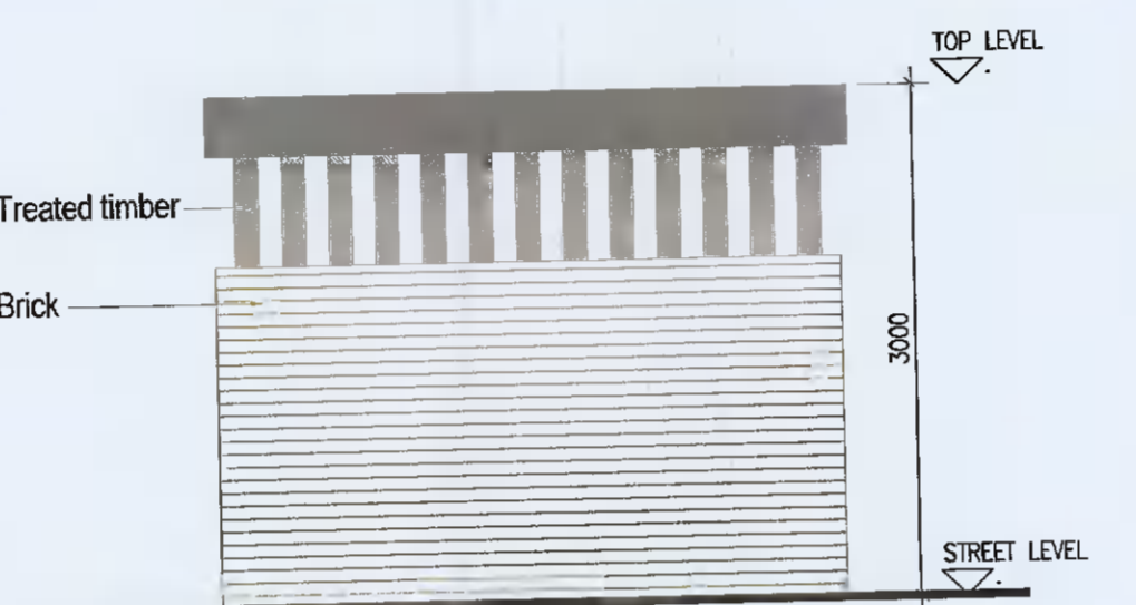
5 Bicycle Store Type 1 Front Elevation Scale 1:50
