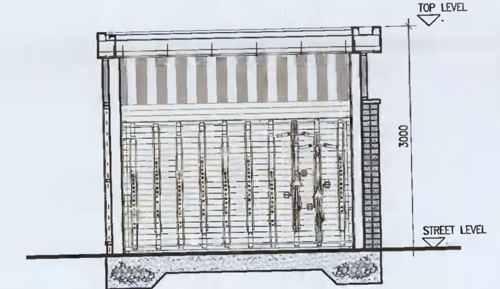
6 Bicycle Store Type 1 Front Elevation Scale 1:50
