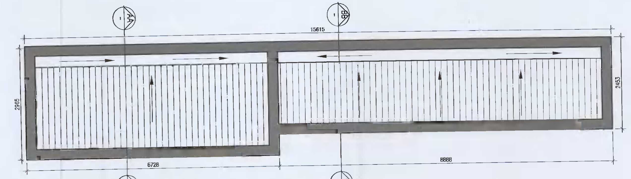
7 Bicycle Store Type 2 Roof Plan Scale 1:50
