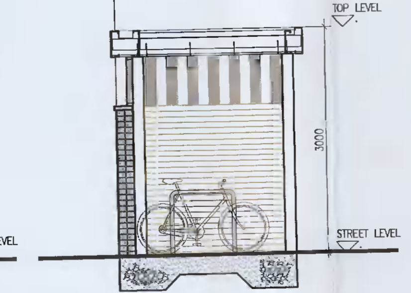
13 Bicycle Store Type 2 Section B Scale 1:50
