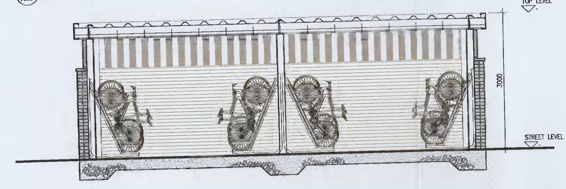
4 Bicycle Store Type 1 Section A Scale 1:50
