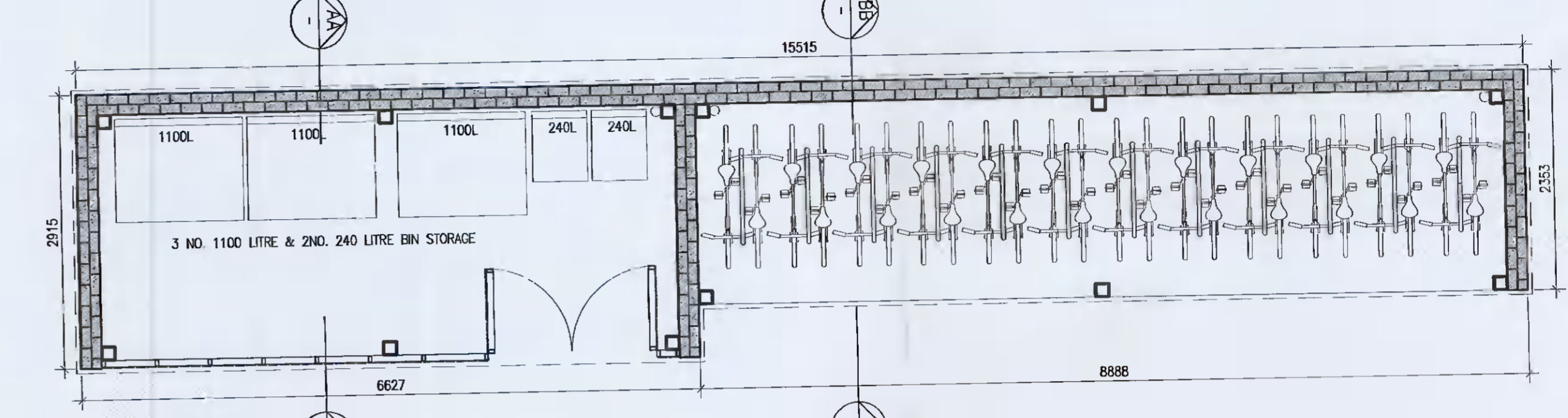
8 Bicycle Store Type 2 Plan Scale 1:50
