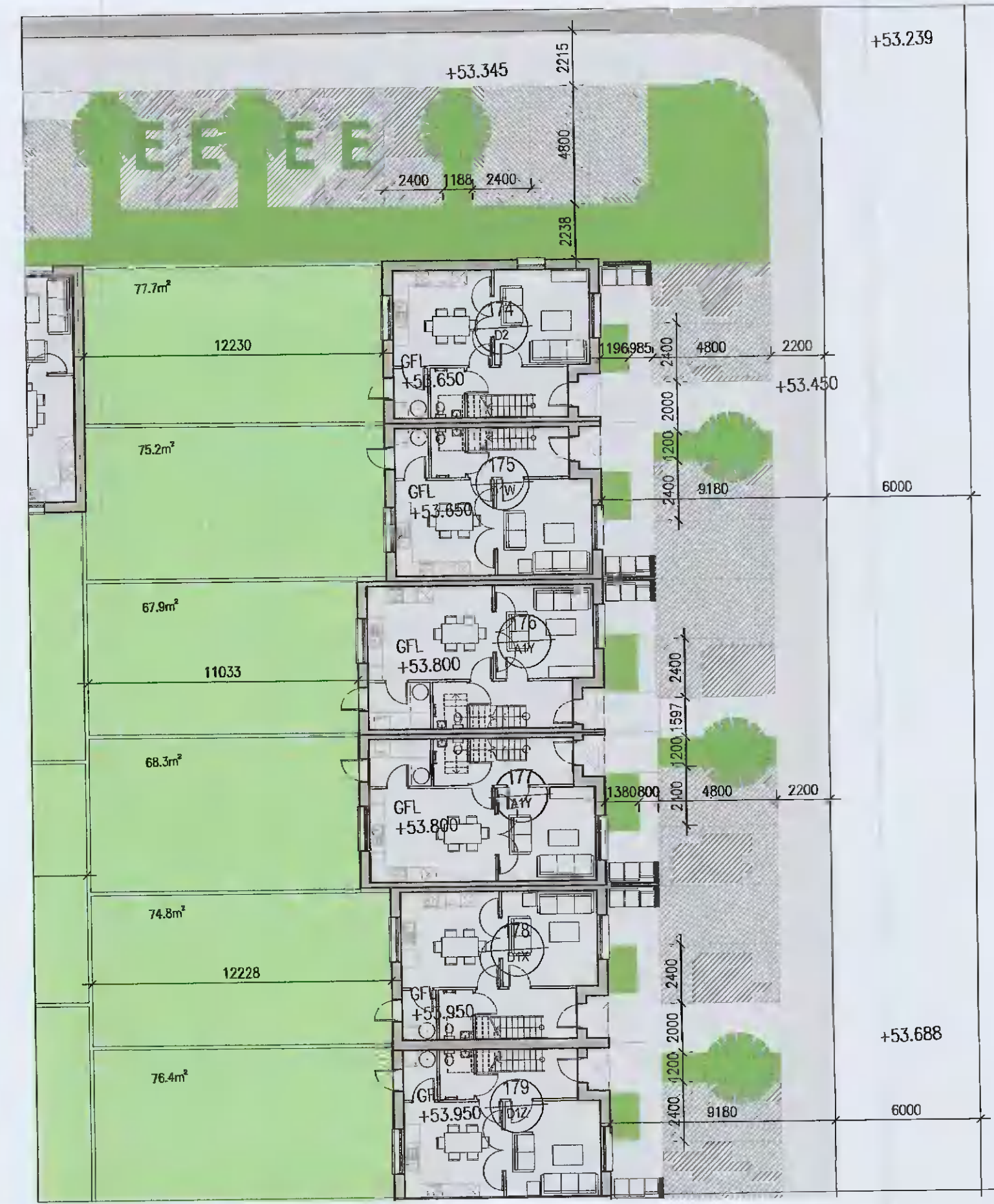
2 Block Plan 2 P301 1:200 @ A1
