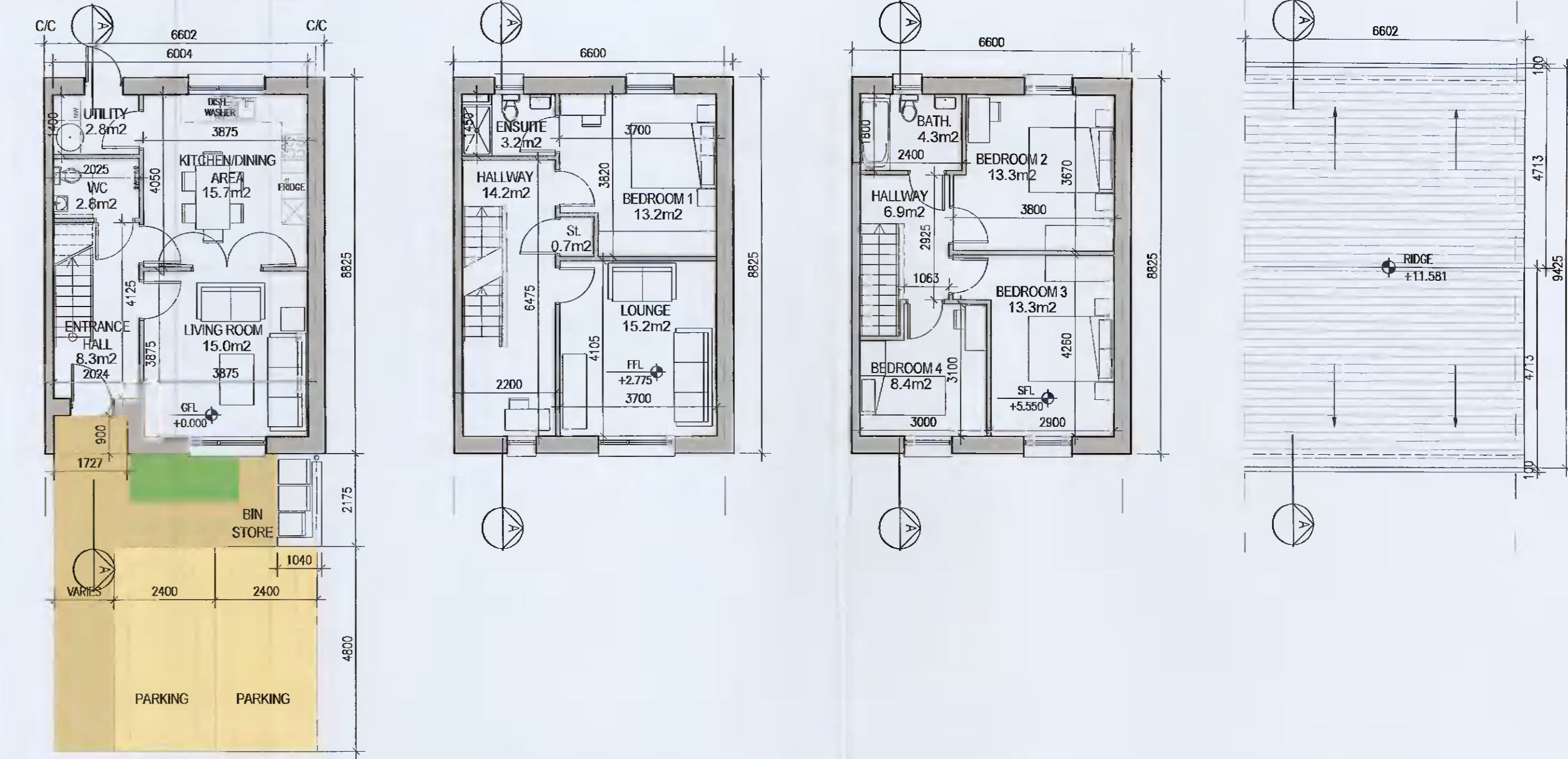
05 Ground Floor Plan 1:100@A1 | 06 First Floor Plan 1:100@A1 | 07 Second Floor Plan 1:100@A1 | 08 Roof Floor Plan 1:100@A1
