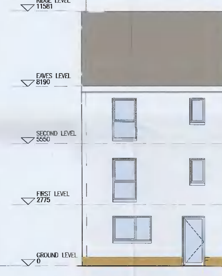
13 Front Elevation 1:100@A1
