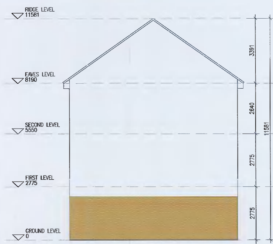
16 Gable Elevation 1:100@A1
