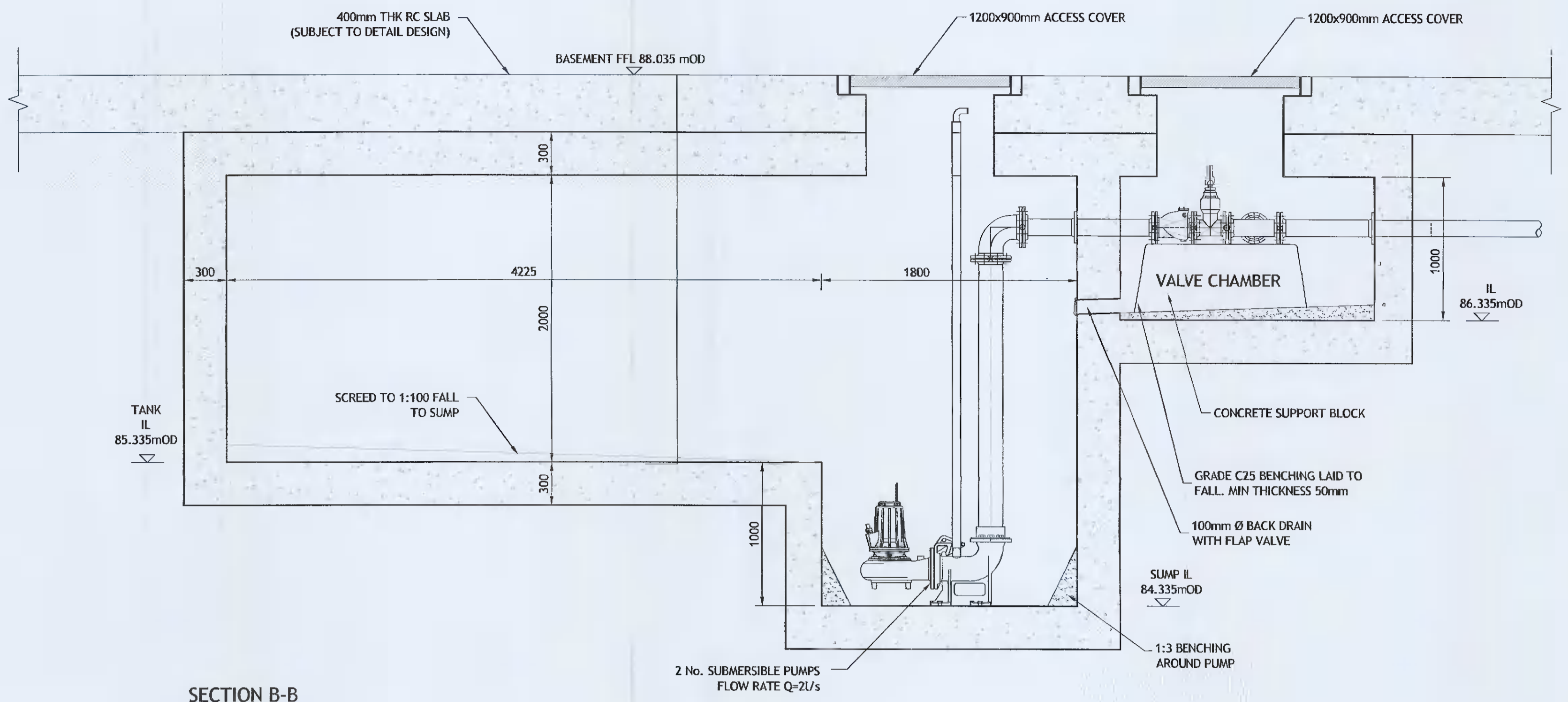
SECTION B-B SCALE 1:25
