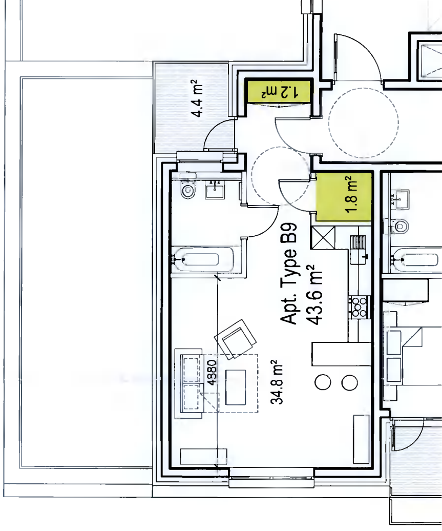
1 Apartment Type B9 PA-616 Scale: 1:100
