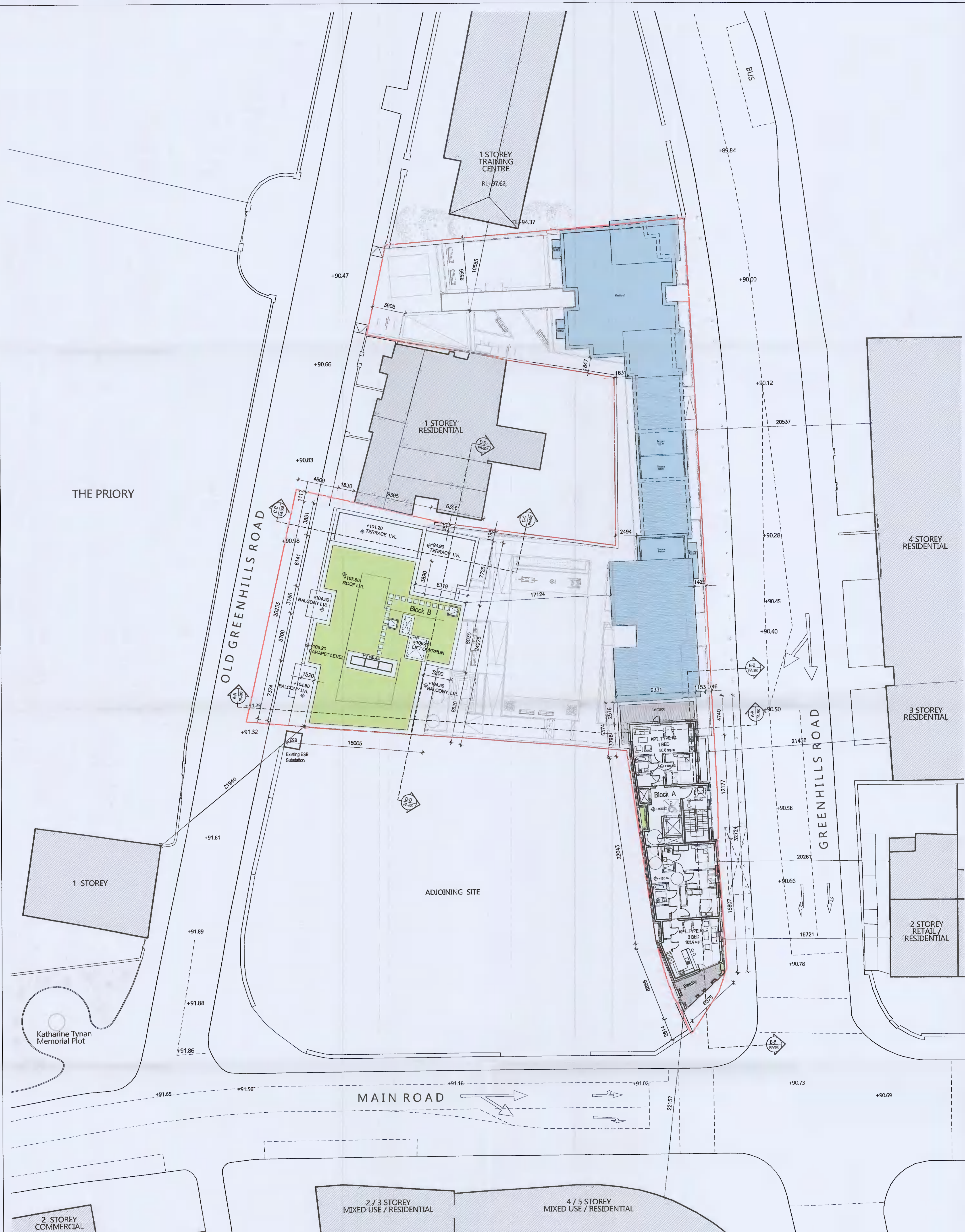
1 PROPOSED FIFTH FLOOR PLAN PA-212 Scale: 1:200
