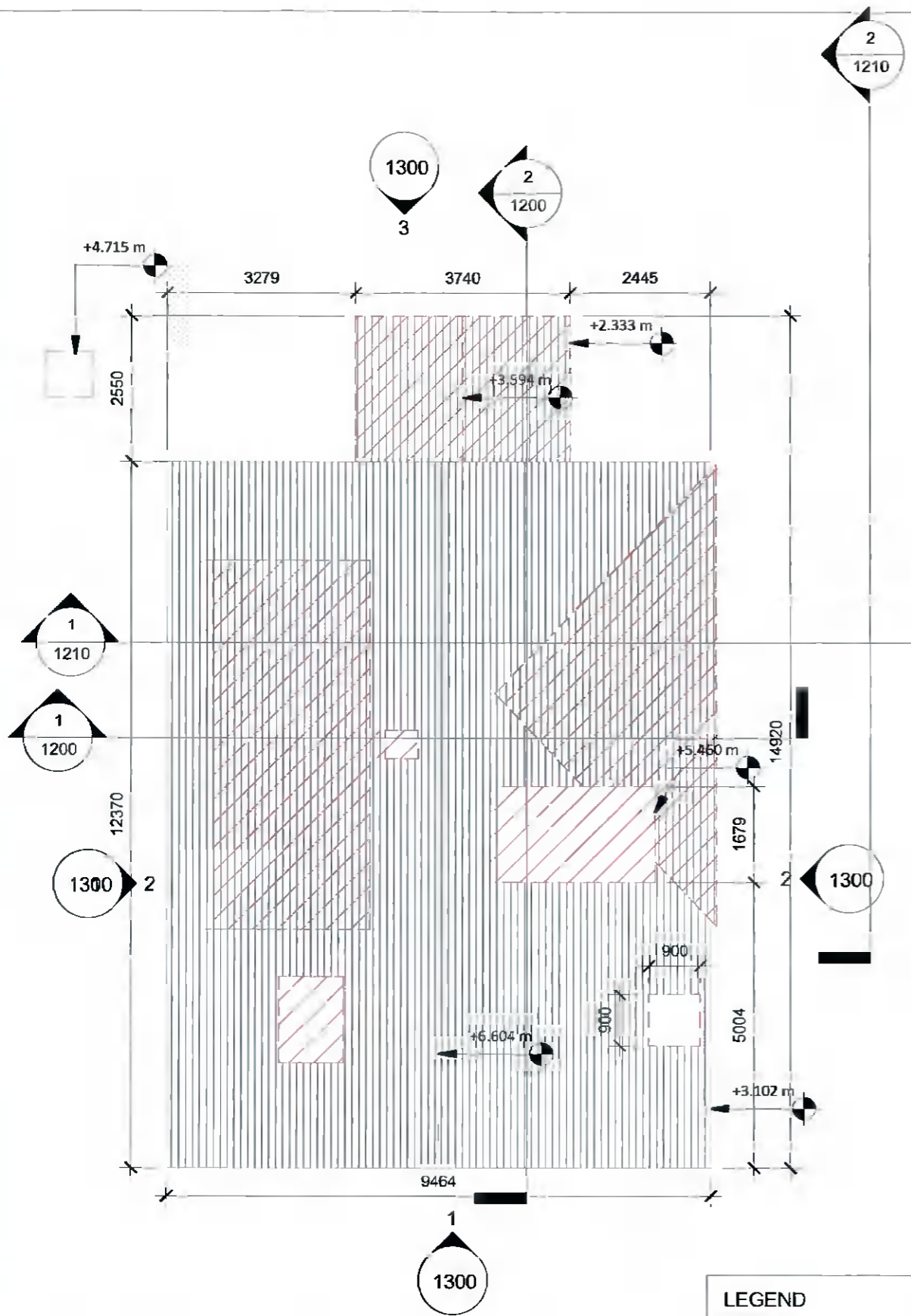
1 Roof plan - Demolition 1 : 100
