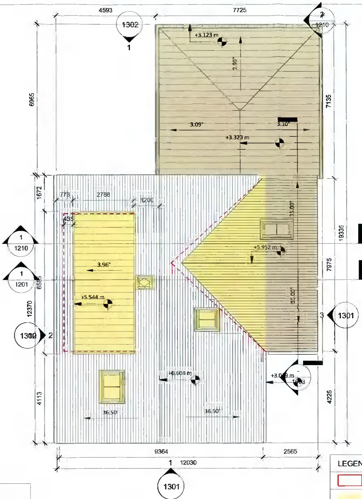
2 Roof plan - Proposed 1 : 100
