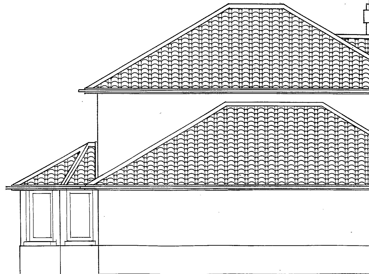
SIDE ELEVATION (15°)
