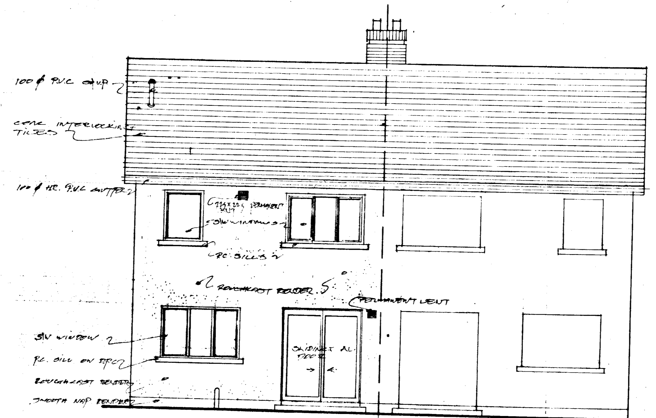
REAR ELEVATION
