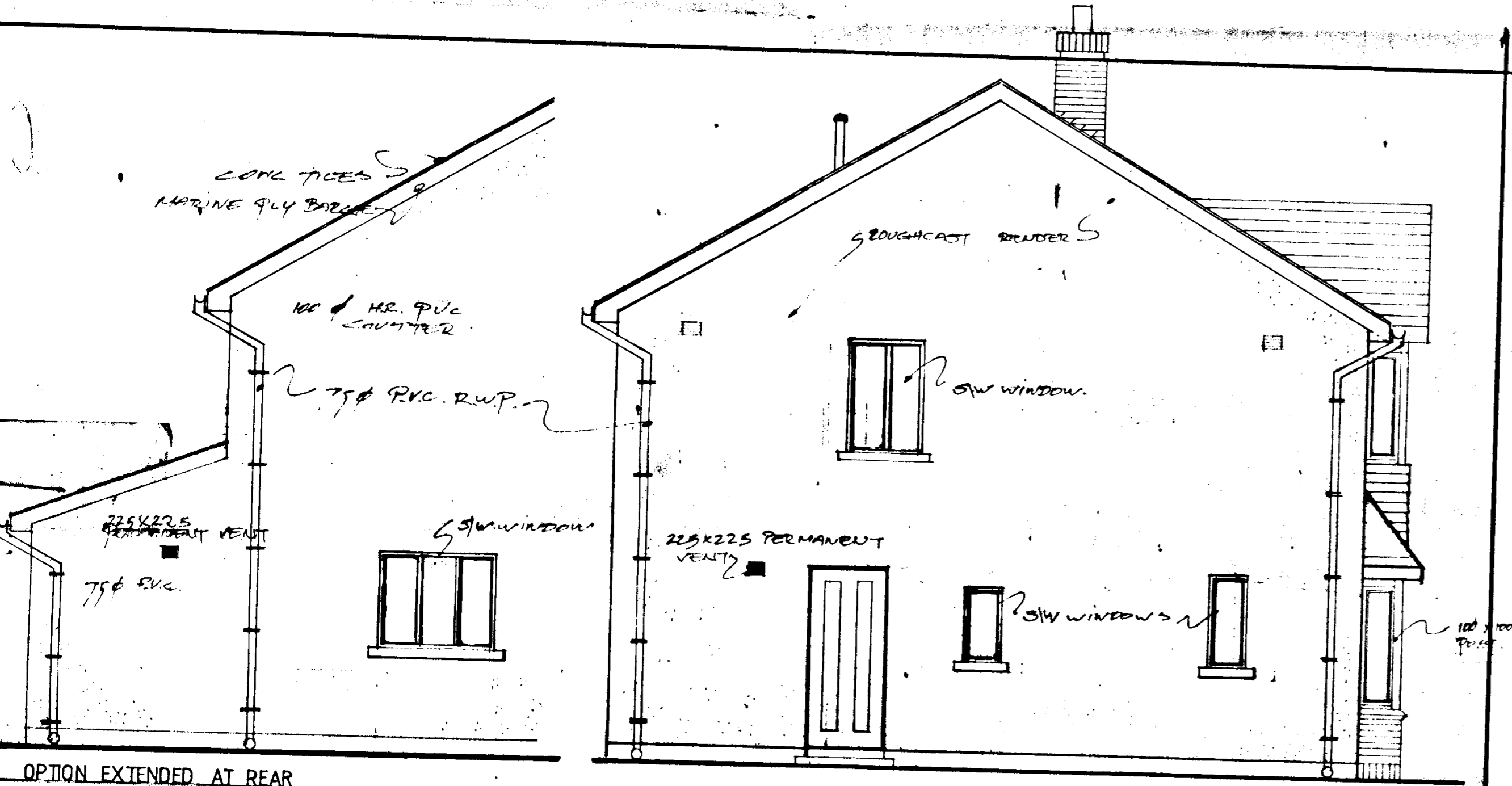
SIDE ELEVATION
