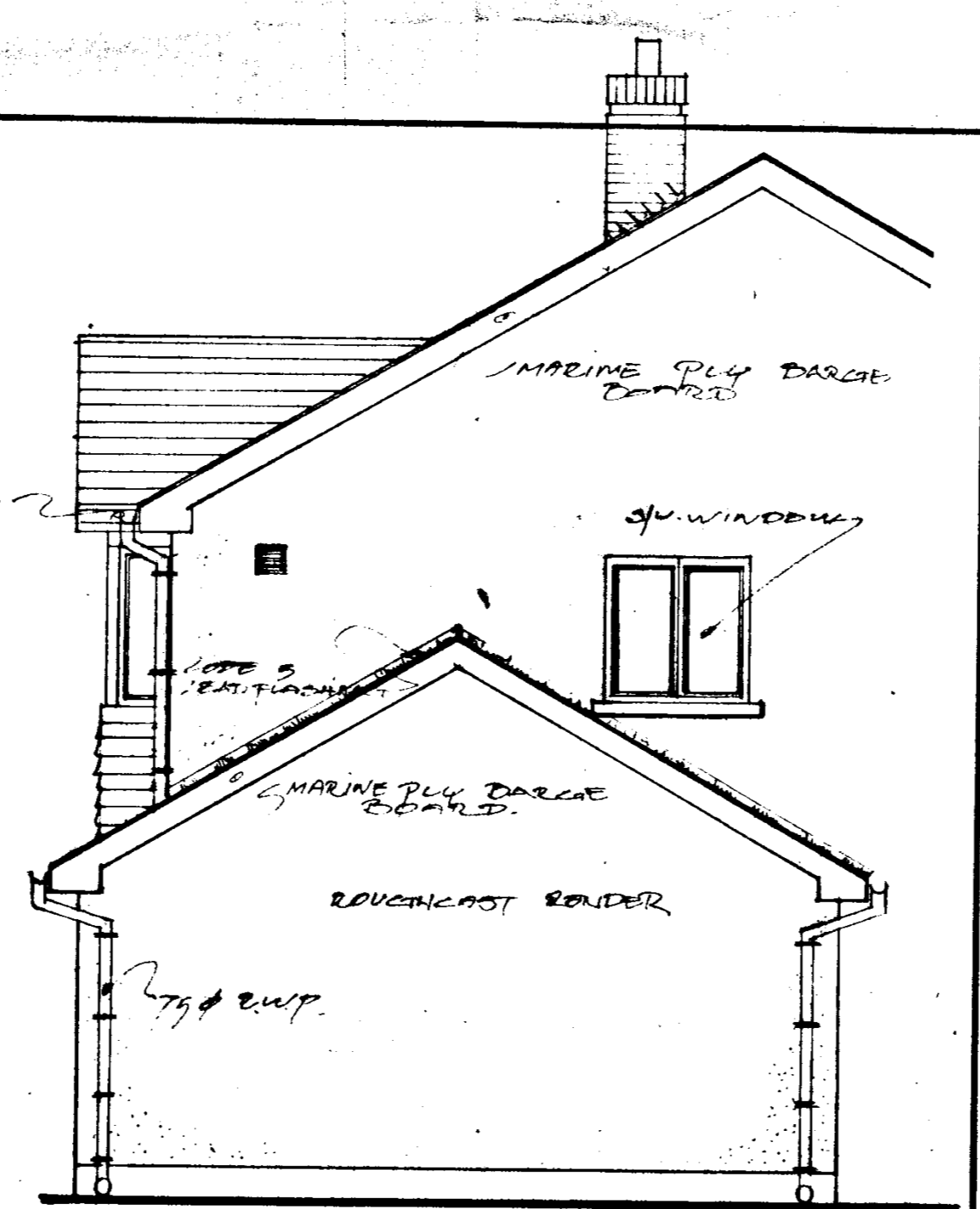
4 BED DETACHED WITH GARAGE
