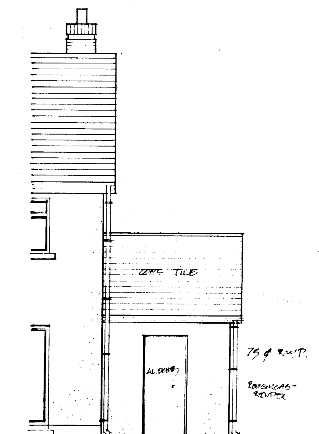
4 BED DETACHED WITH GARAGE
