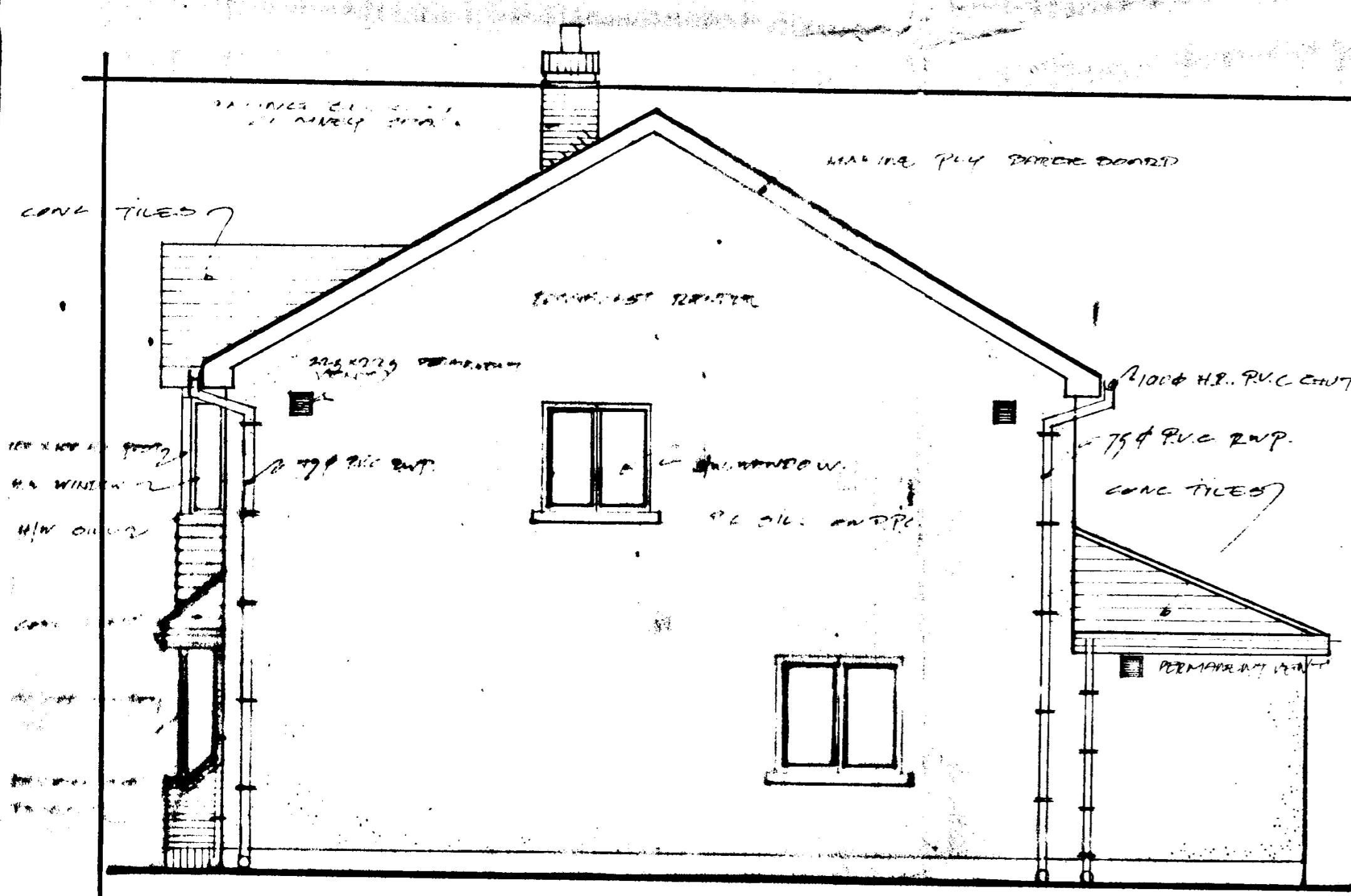
SIDE ELEVATION
