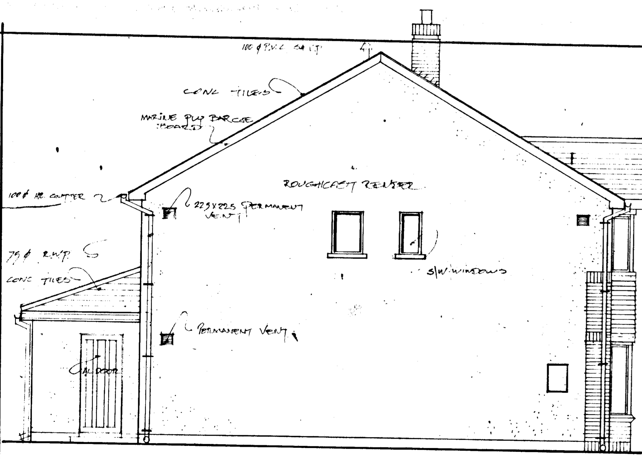
SIDE ELEVATION
