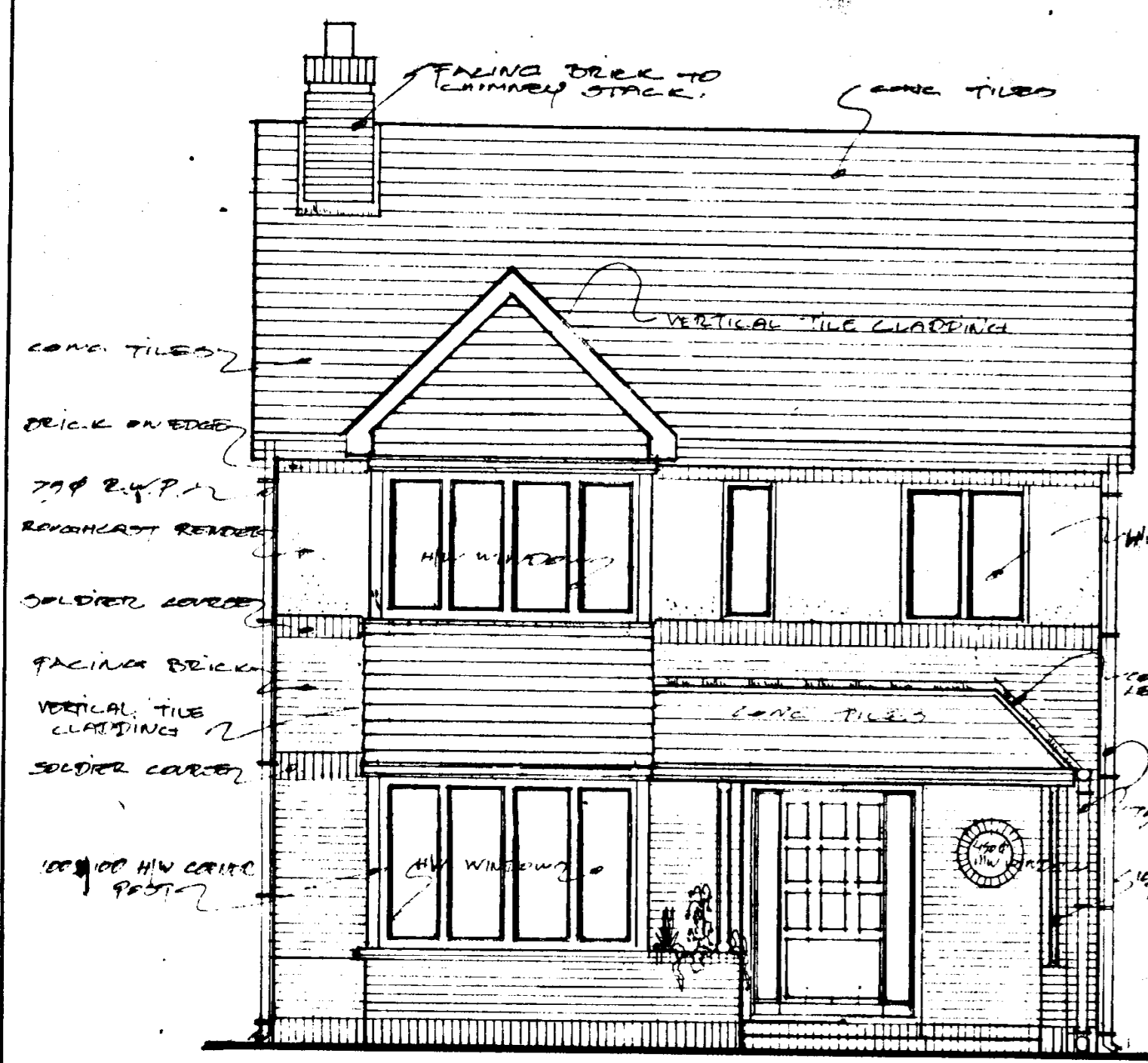
FRONT ELEVATION
