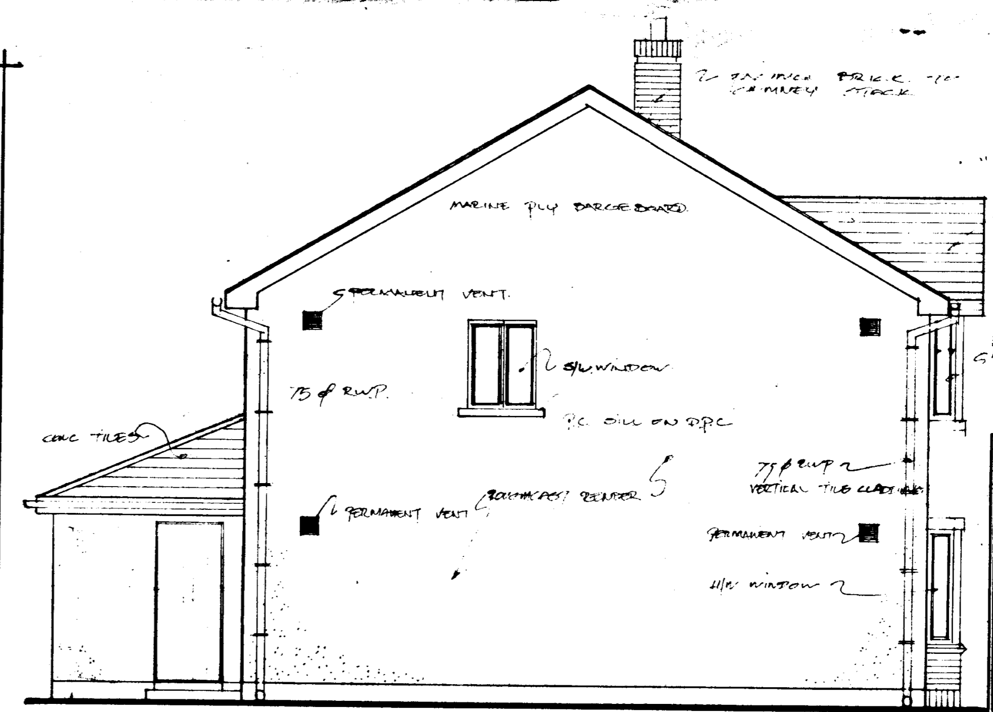
SIDE ELEVATION
