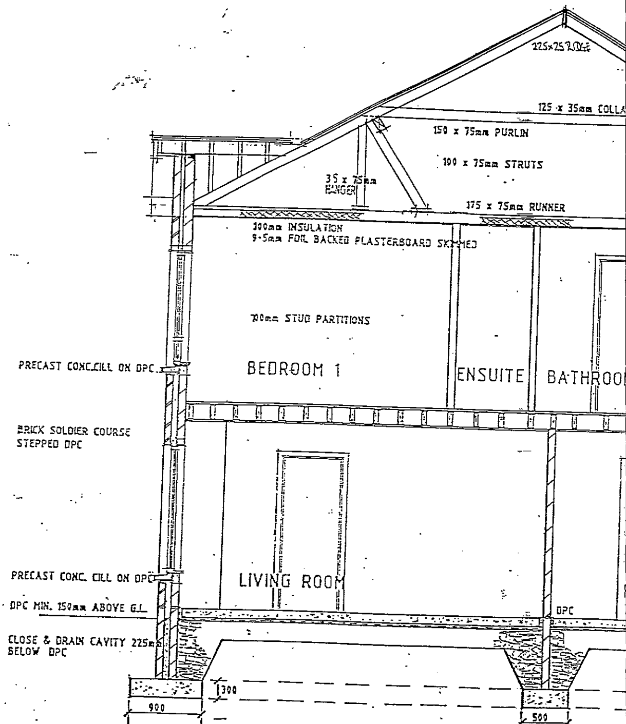
TYPICAL SECTION
